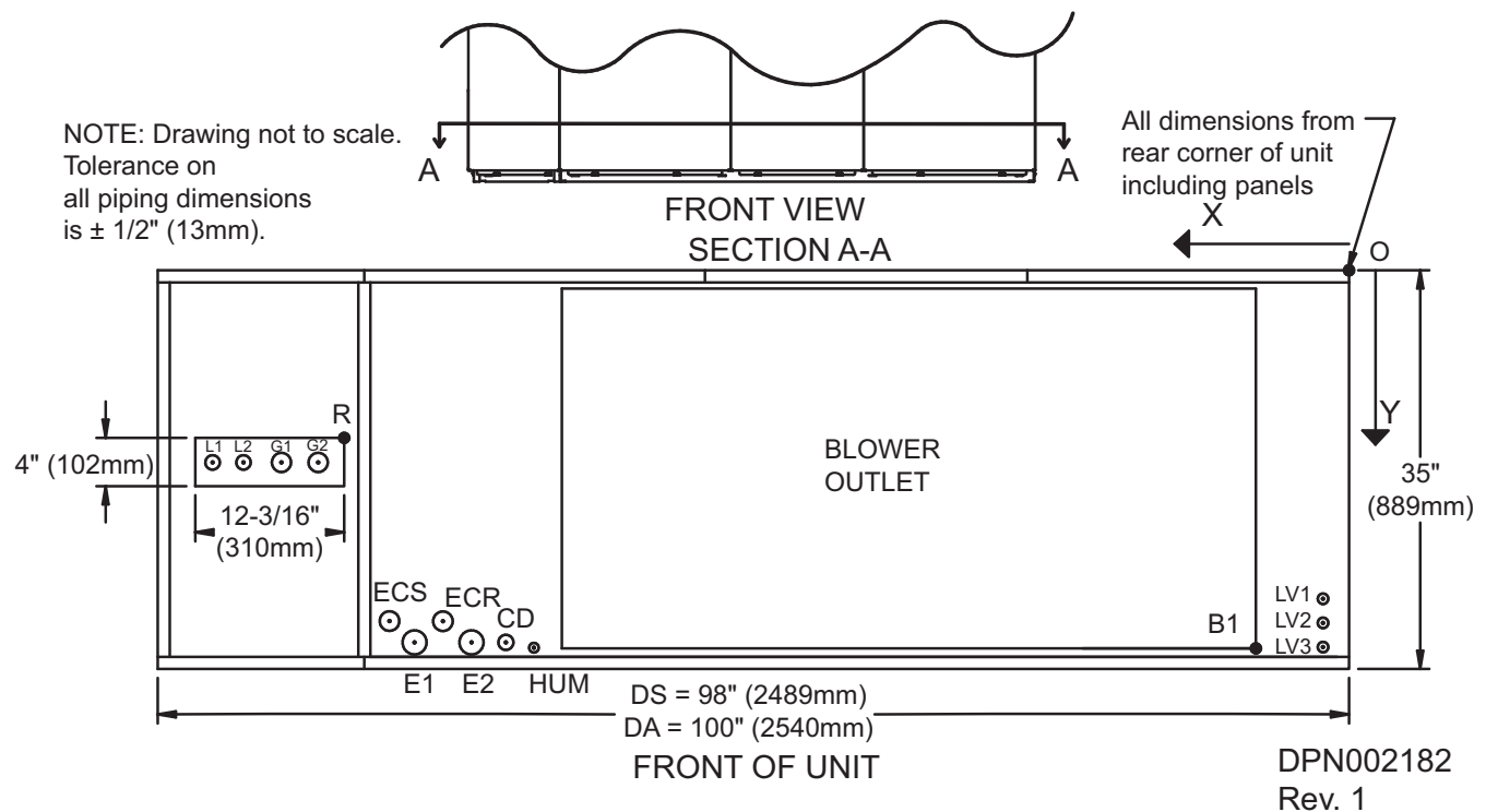
Figure 83 Primary connection locations—downflow, air-Cooled, 53-77kW (15-22 ton) with scroll *** compressor models, with EC fan
