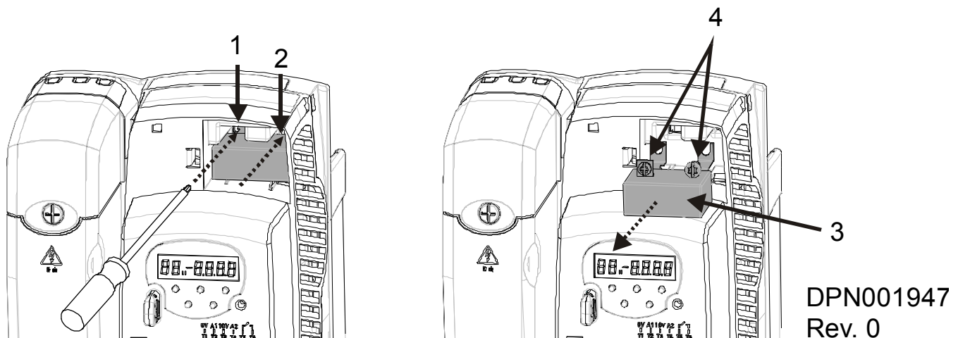
Figure 66 Figure bb Disconnecting EMC filter for operation with Delta-connected power Type 2 inverters
