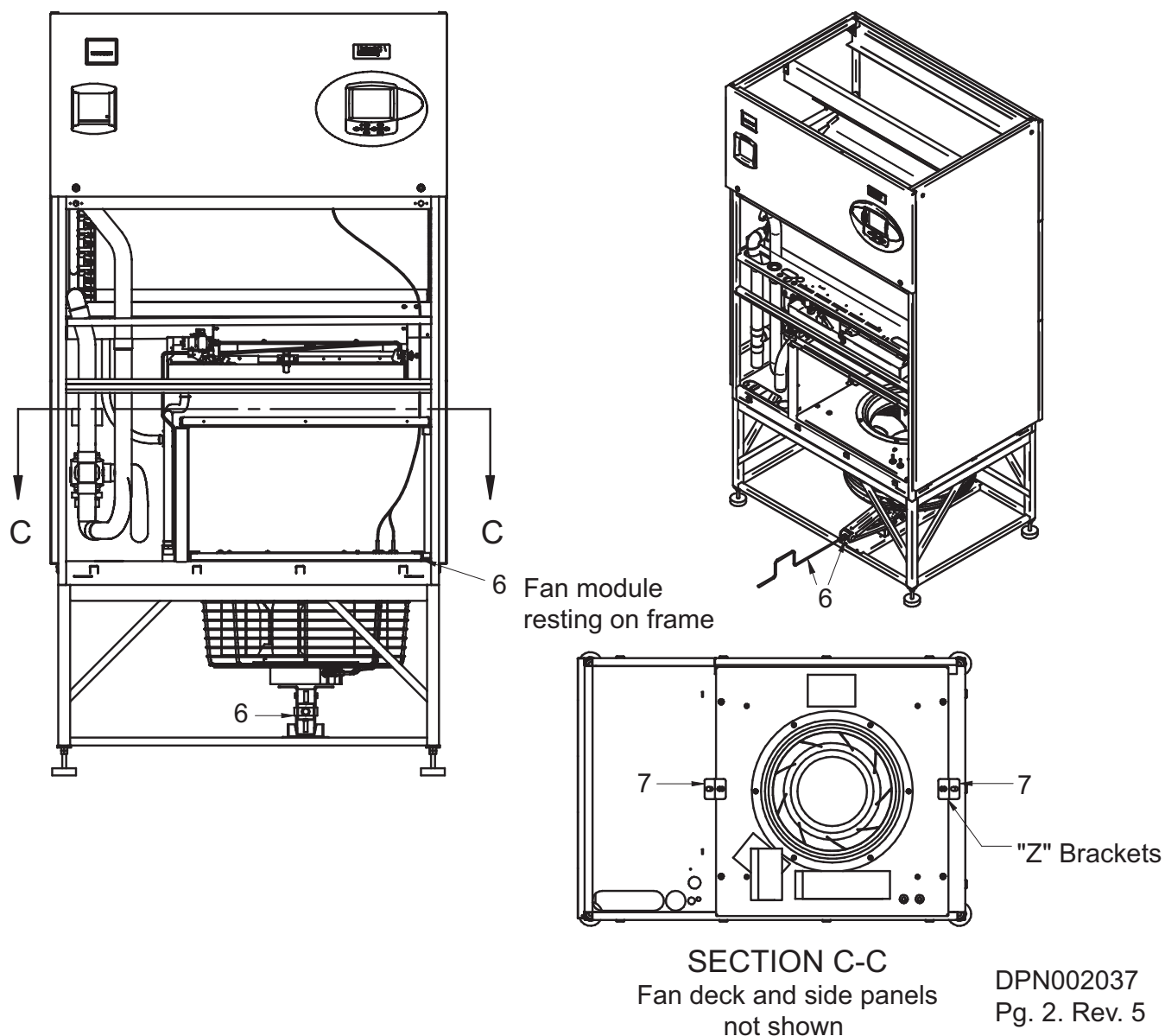
Figure 40 Lowering EC fans into floor stand, Steps 7 through 9
