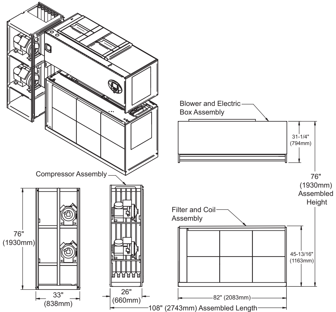
Figure 57 Component dimensions—upflow water/glycol/GLYCOOL 53-77kw (15-22 ton), all compressor models
