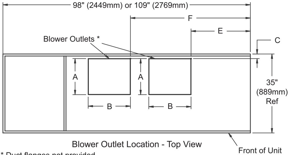
Figure 28 Blower outlet and deck dimensions—upflow, 53-77kW (15-22 ton) with forward-curved fans
