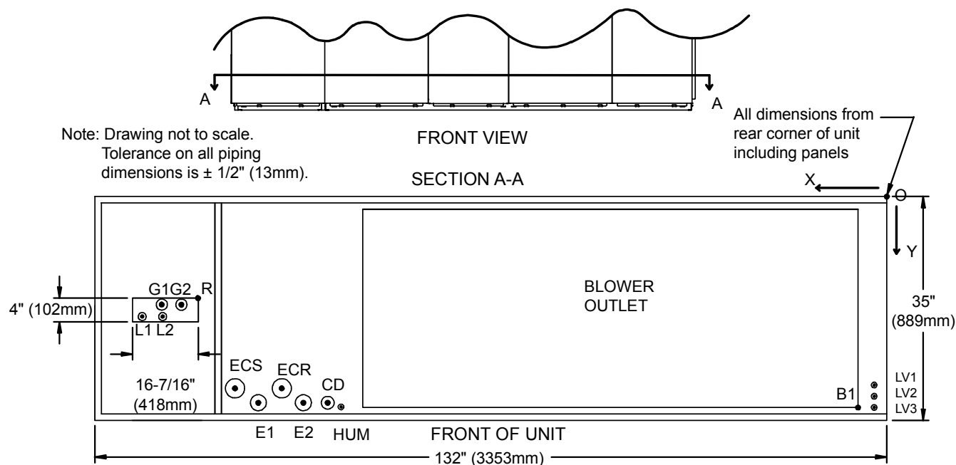
Figure 87 Primary connection locations—downflow, air-cooled, 105kW (30 ton), all compressor *** models, with EC fan
