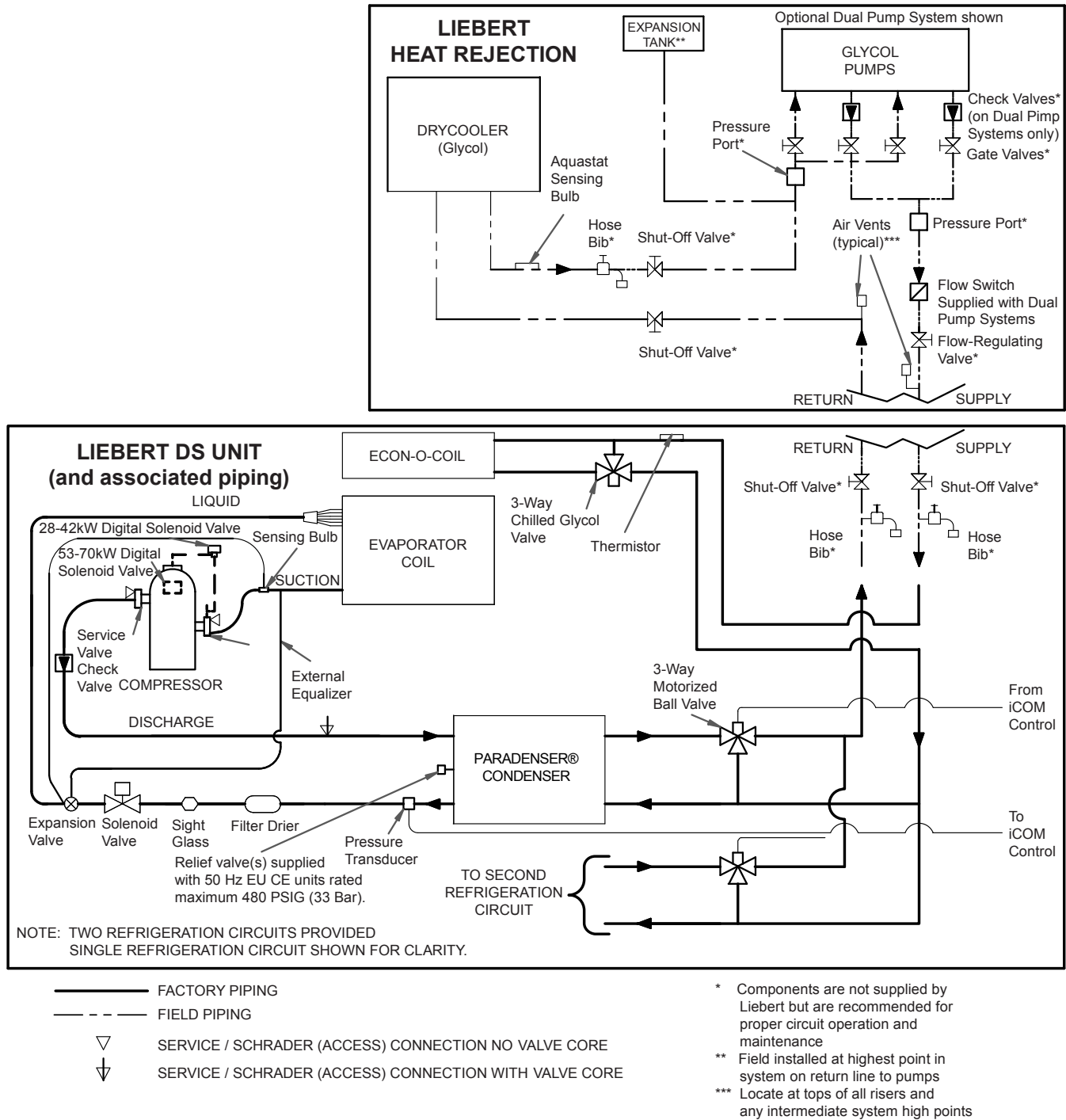
Figure 75 GLYCOOL with digital scroll compressor models
