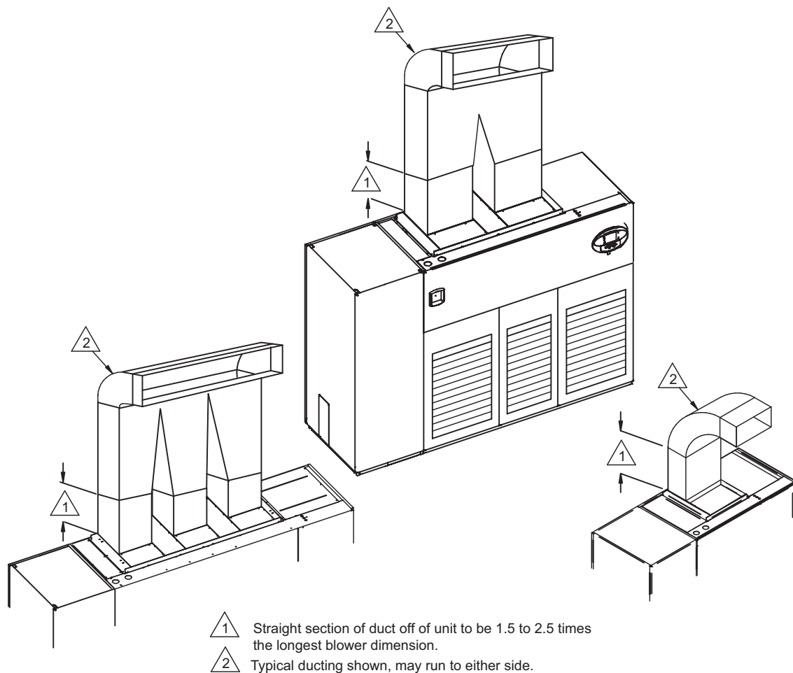
Figure 5 Upflow ducting configurations
