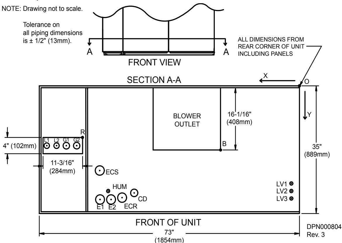
Figure 78 Primary connection locations—downflow, air-Cooled, 28-42kW (8-12 ton) with scroll compressor models
