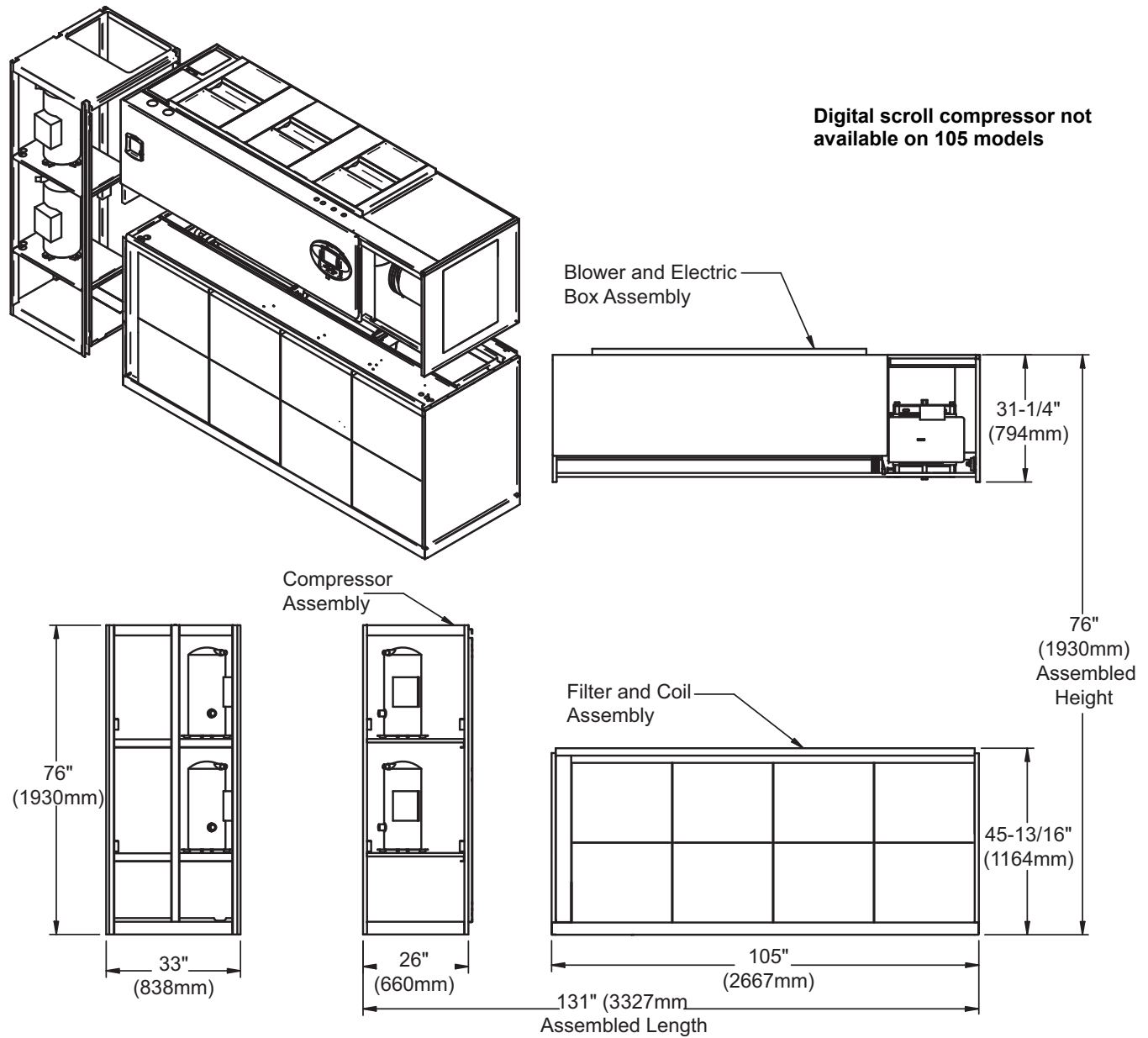
Figure 59 Component dimensions—upflow, air-cooled, 105kW (30 ton), scroll/digital scroll compressor models
