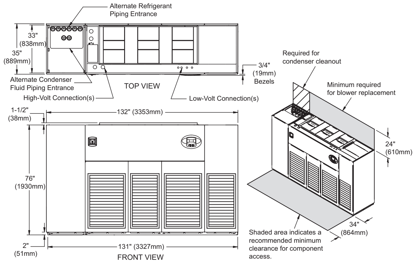
Figure 21 Cabinet and floor planning dimensions—upflow water/glycol/GLYCOOL 105kW (30 ton), all models
