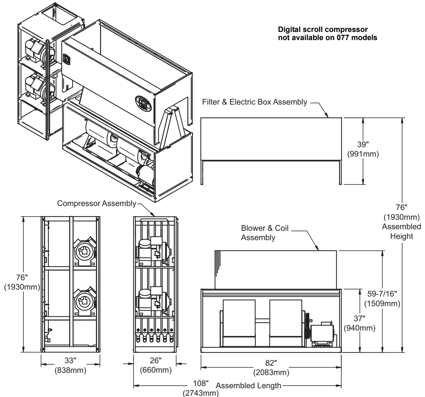
Figure 48 Component dimensions—downflow water/glycol, GLYCOOL, 53-77kW (15-22 ton), all compressor models; forward-curved and EC fan
