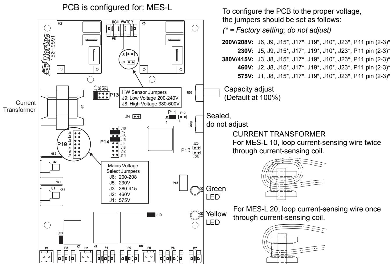
Figure 107 Circuit board diagram
