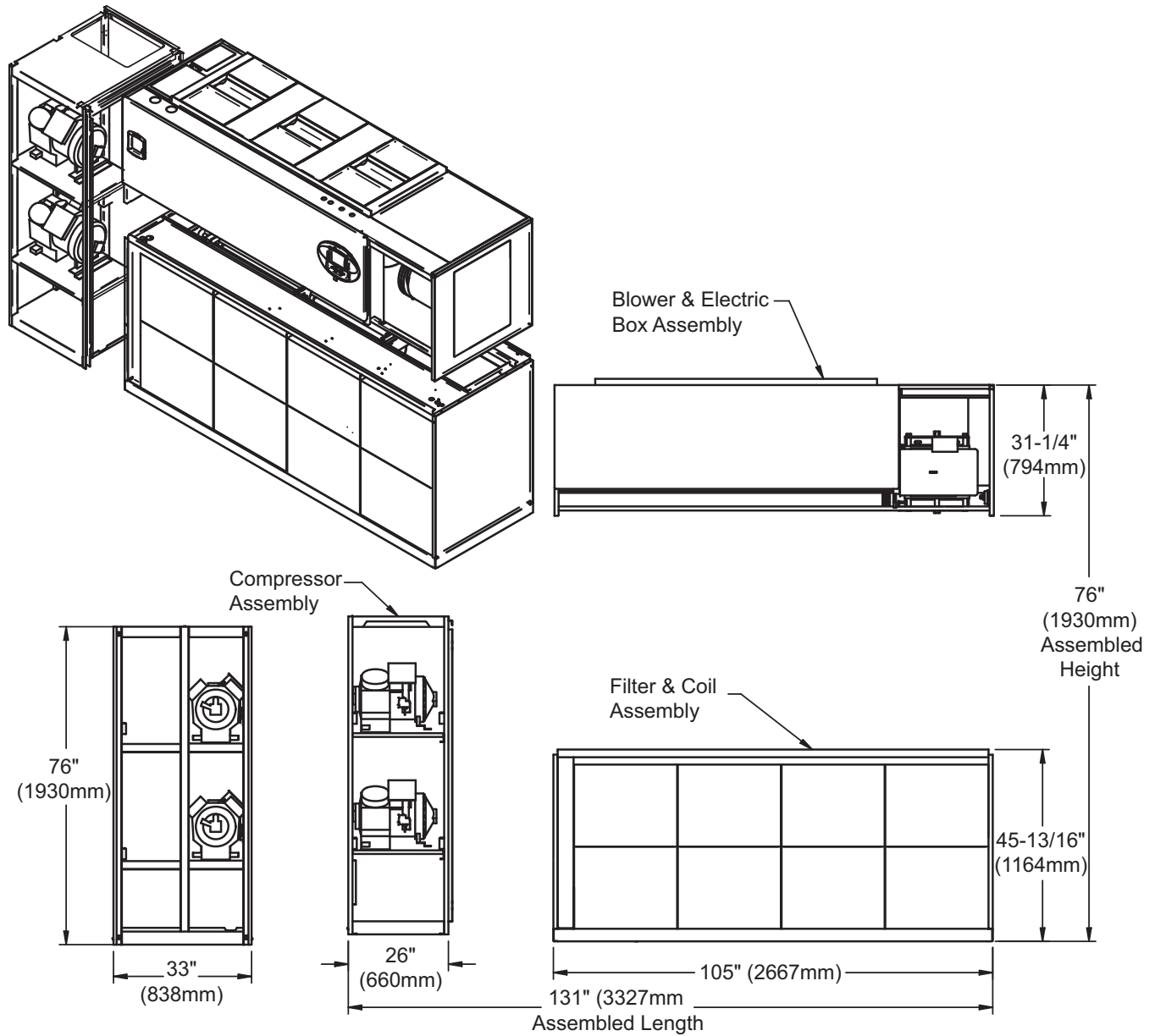
Figure 58 Component dimensions—upflow, air-cooled, 105kW (30 ton), semi-hermetic compressor models
