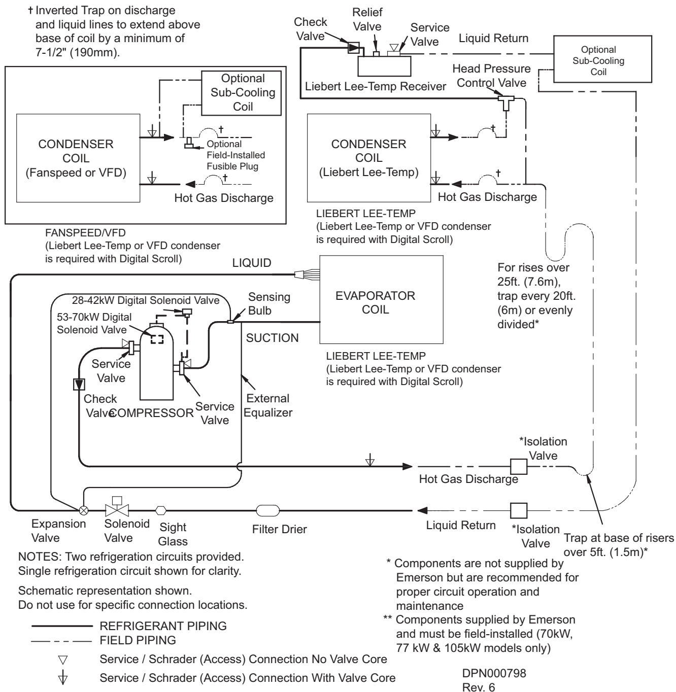
Figure 69 Piping schematic—air-cooled, scroll compressor models
