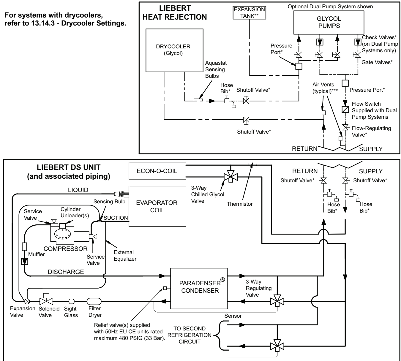
Figure 72 Piping schematic—GLYCOOL semi-hermetic compressor models
