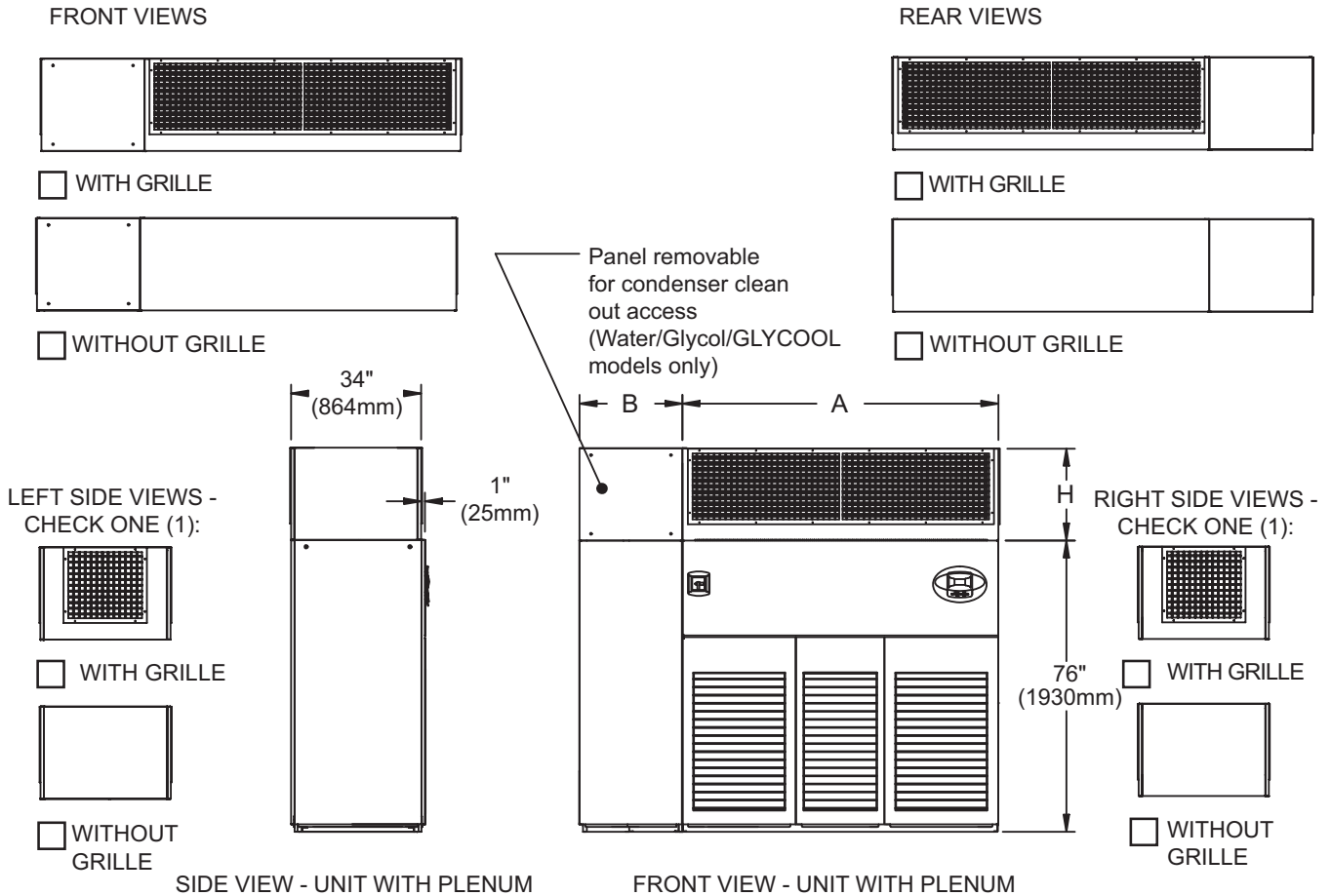
Figure 31 Upflow unit plenum dimensions
