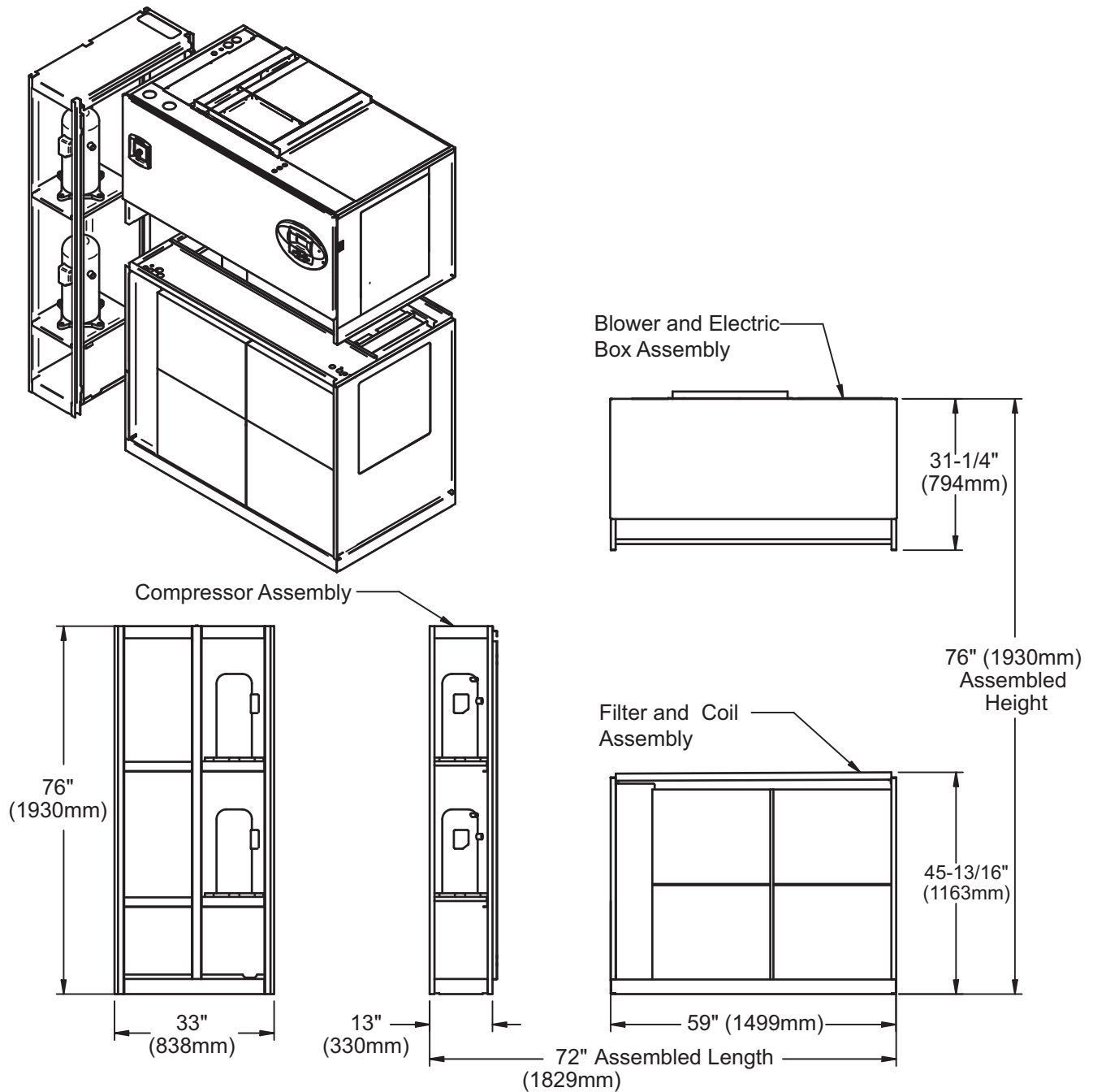
Figure 53 Component dimensions—upflow, air-cooled, 28-42kW (8-12 ton), scroll/digital scroll compressor models
