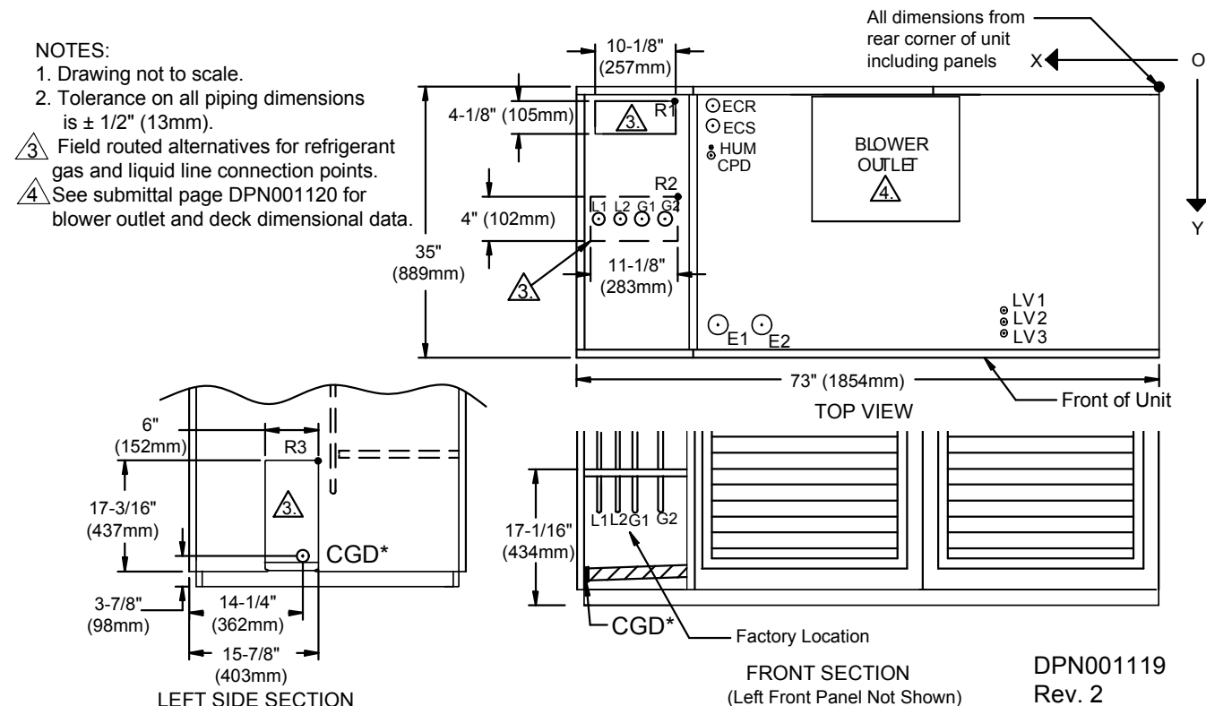
Figure 91 Primary connection locations—upflow, air-Cooled, 28-42kW (8-12 ton), semi-hermetic compressor models
