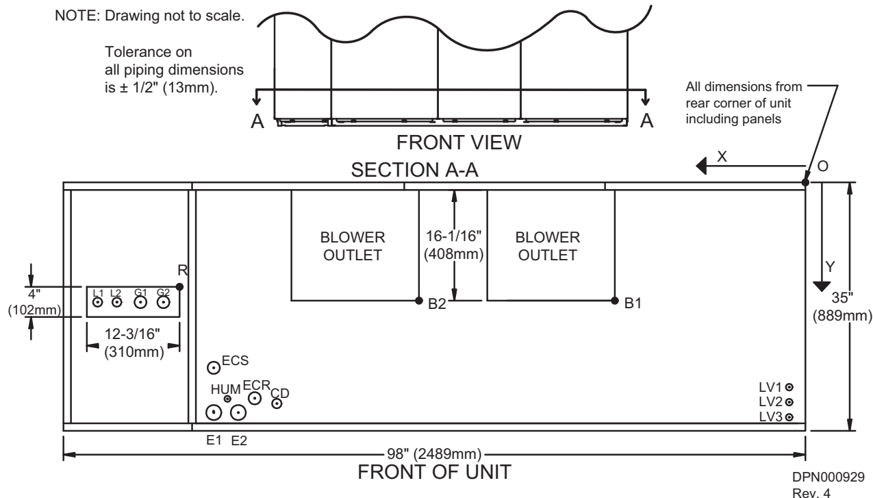
Figure 82 Primary connection locations—downflow, air-Cooled, 53-77kW (15-22 ton) with scroll *** compressor models
