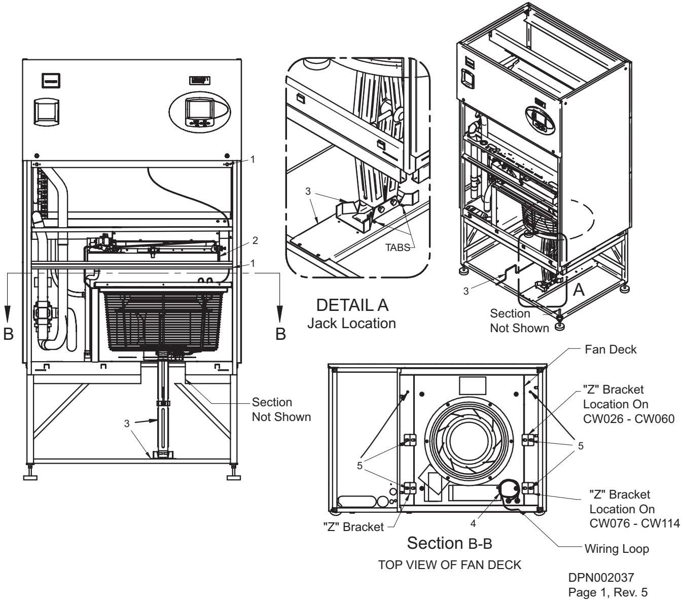
Figure 39 Lowering EC fans into floor stand, Steps 1 through 6
