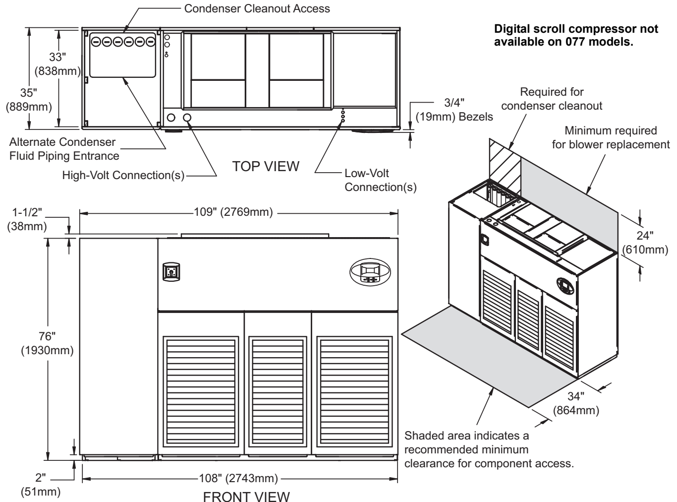
Figure 19 Cabinet and floor planning dimensions—upflow, water/glycol/GLYCOOL, 53-77kW (15-22 ton), all compressor models
