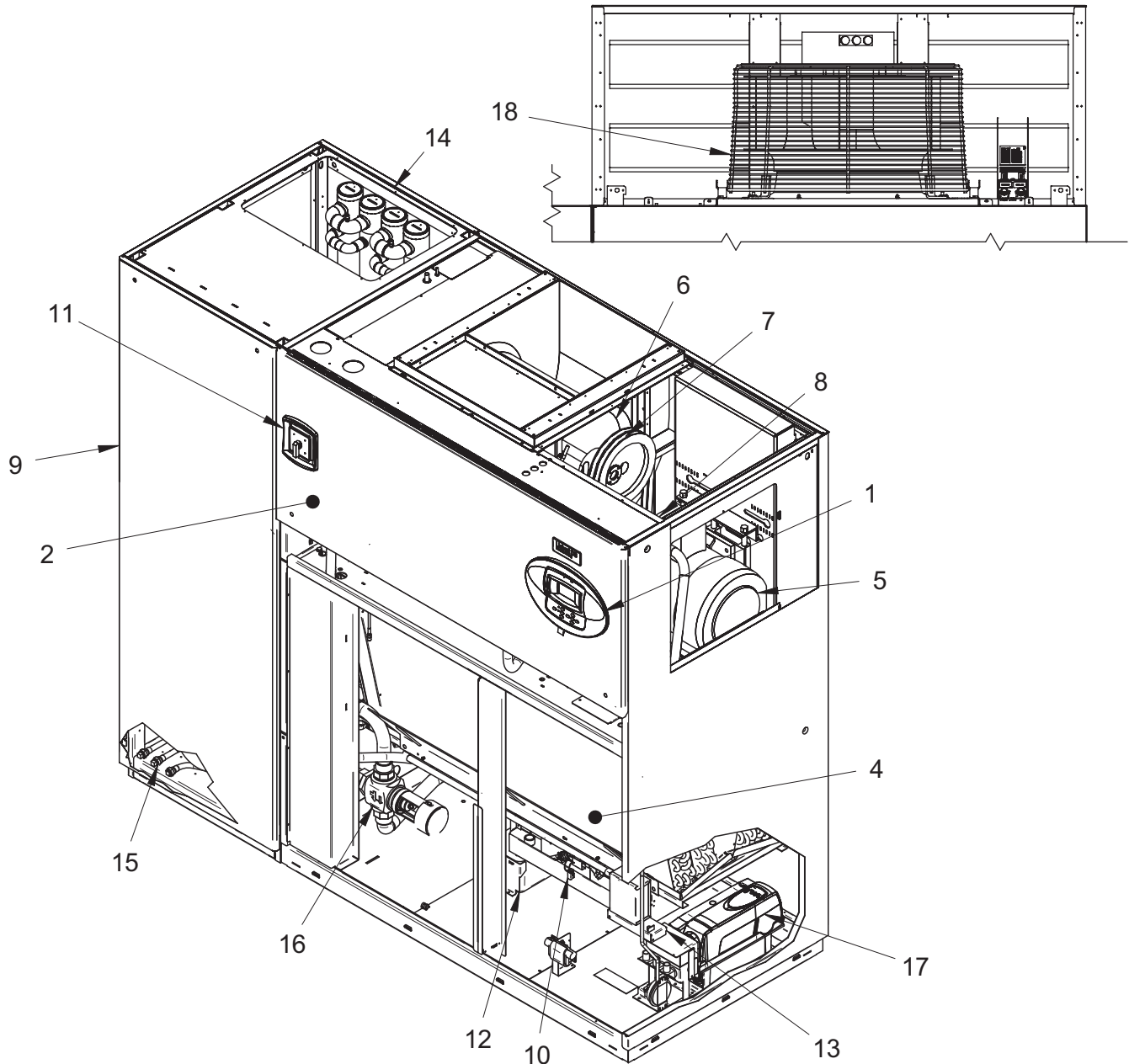
Figure 2 Upflow model component locations
