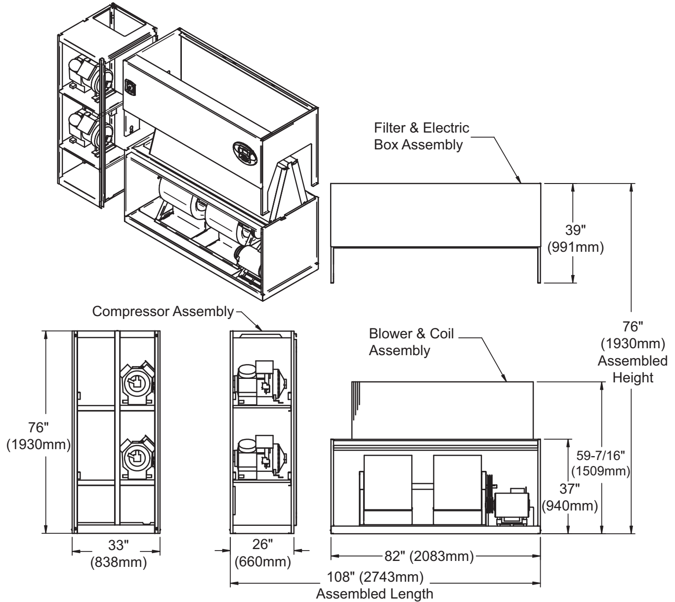
Figure 46 Component dimensions—downflow, air-cooled, 53-77kW (15-22 ton), semi-hermetic compressor models; forward-curved and EC fan
