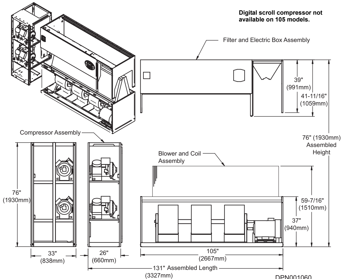
Figure 51 Component dimensions—downflow, water/glycol/GLYCOOL, 105kW (30 ton), forward-curved and EC fan, all compressor models; forward-curved and EC fan
