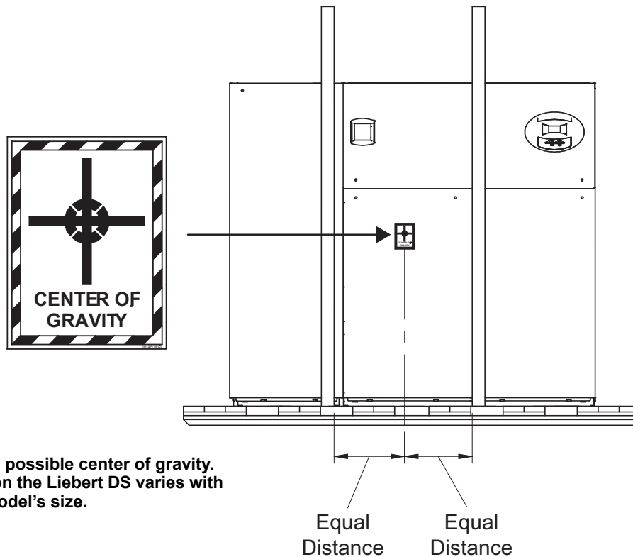
Figure 36 Locate center of gravity marker and place slings
