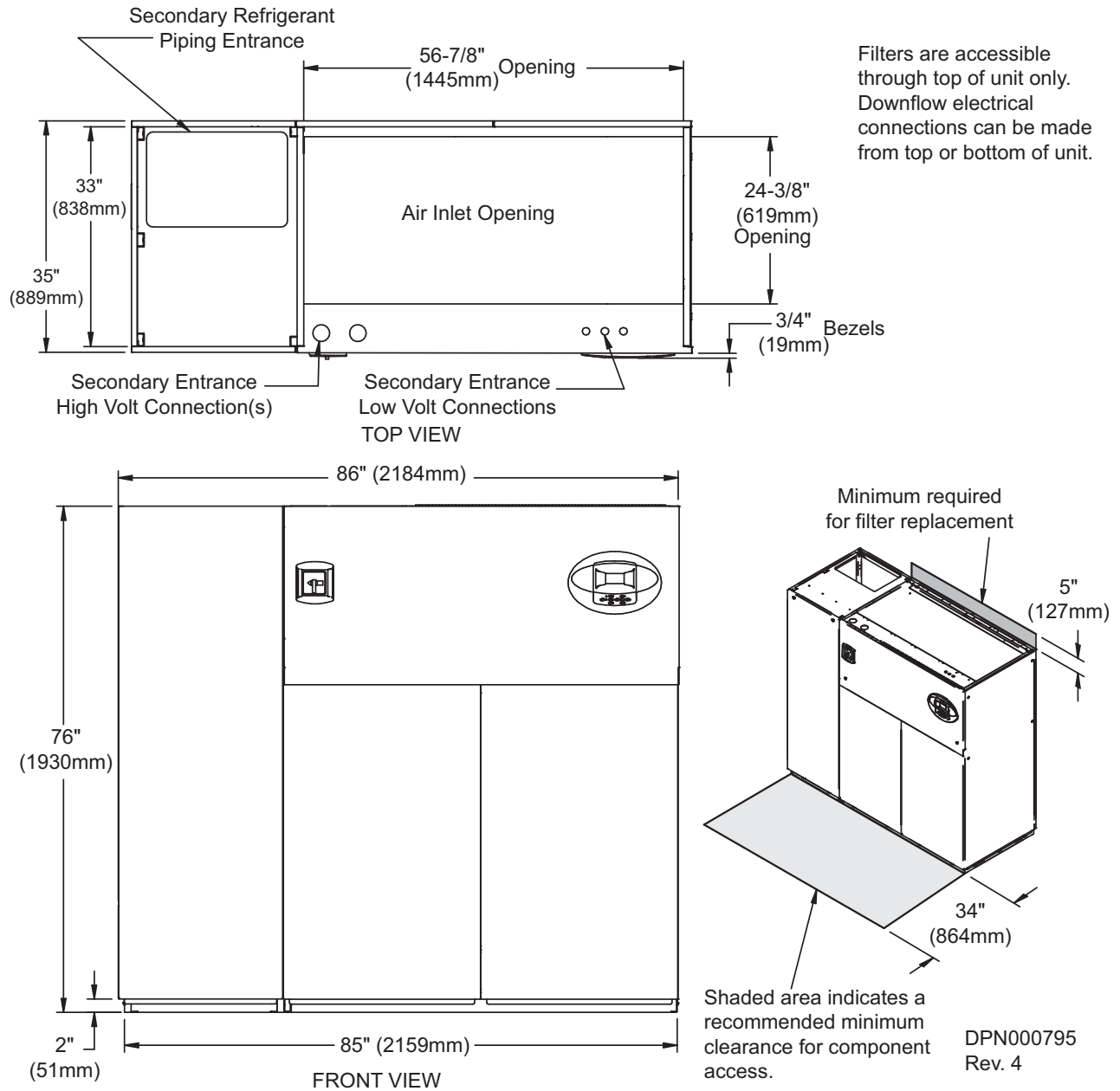
Figure 6 Cabinet and floor planning dimensions—downflow, air-cooled, 28-42kW (8-12 ton), semi-hermetic compressor models
