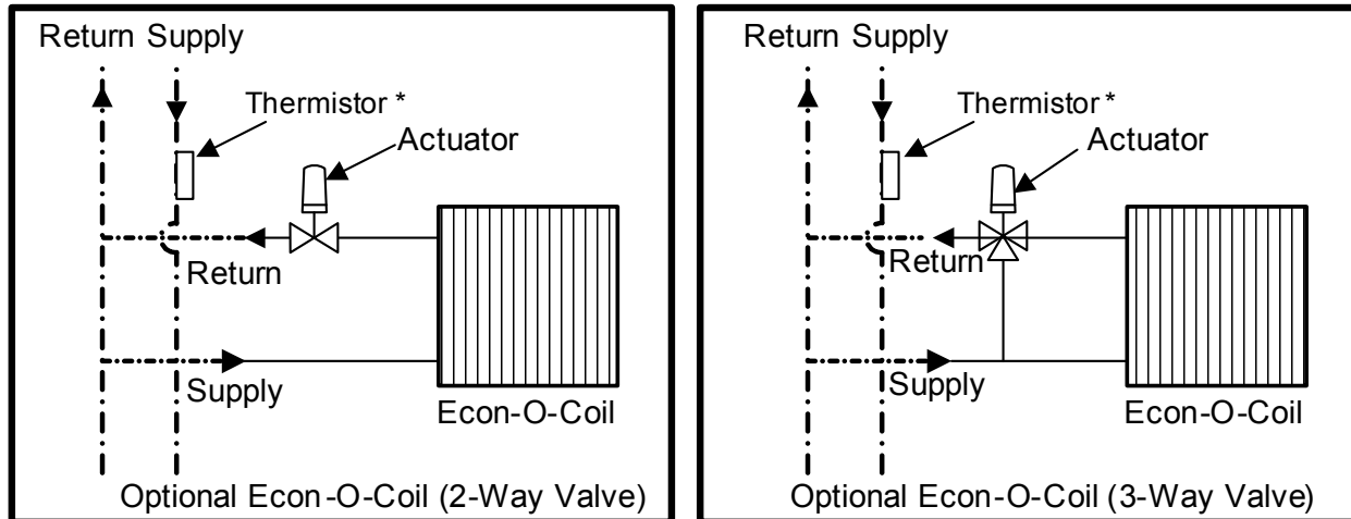
Figure 76 Optional piping schematic for Econ-O-Coil
