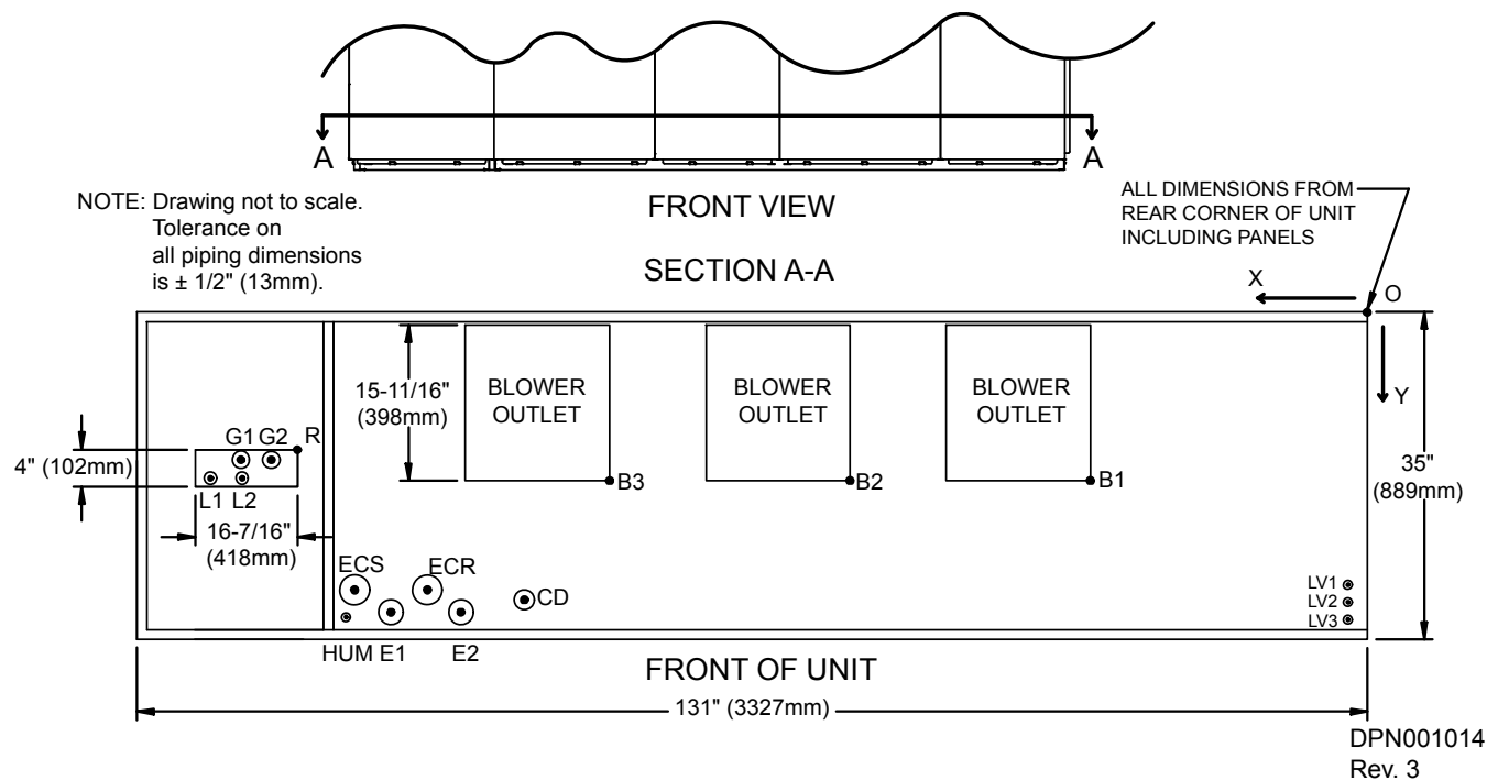
Figure 86 Primary connection locations—downflow, air-cooled, 105kW (30 ton), all compressor*** models
