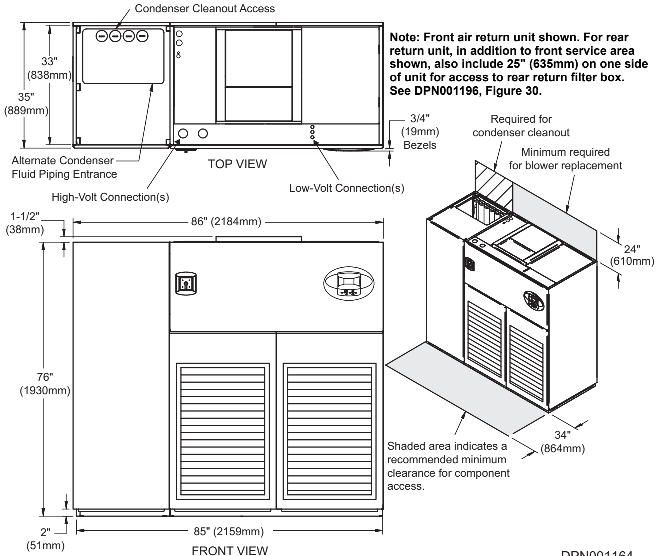
Figure 16 Cabinet and floor planning dimensions—upflow, water/glycol/GLYCOOL, 28-42kW (8-12 ton), all compressor models
