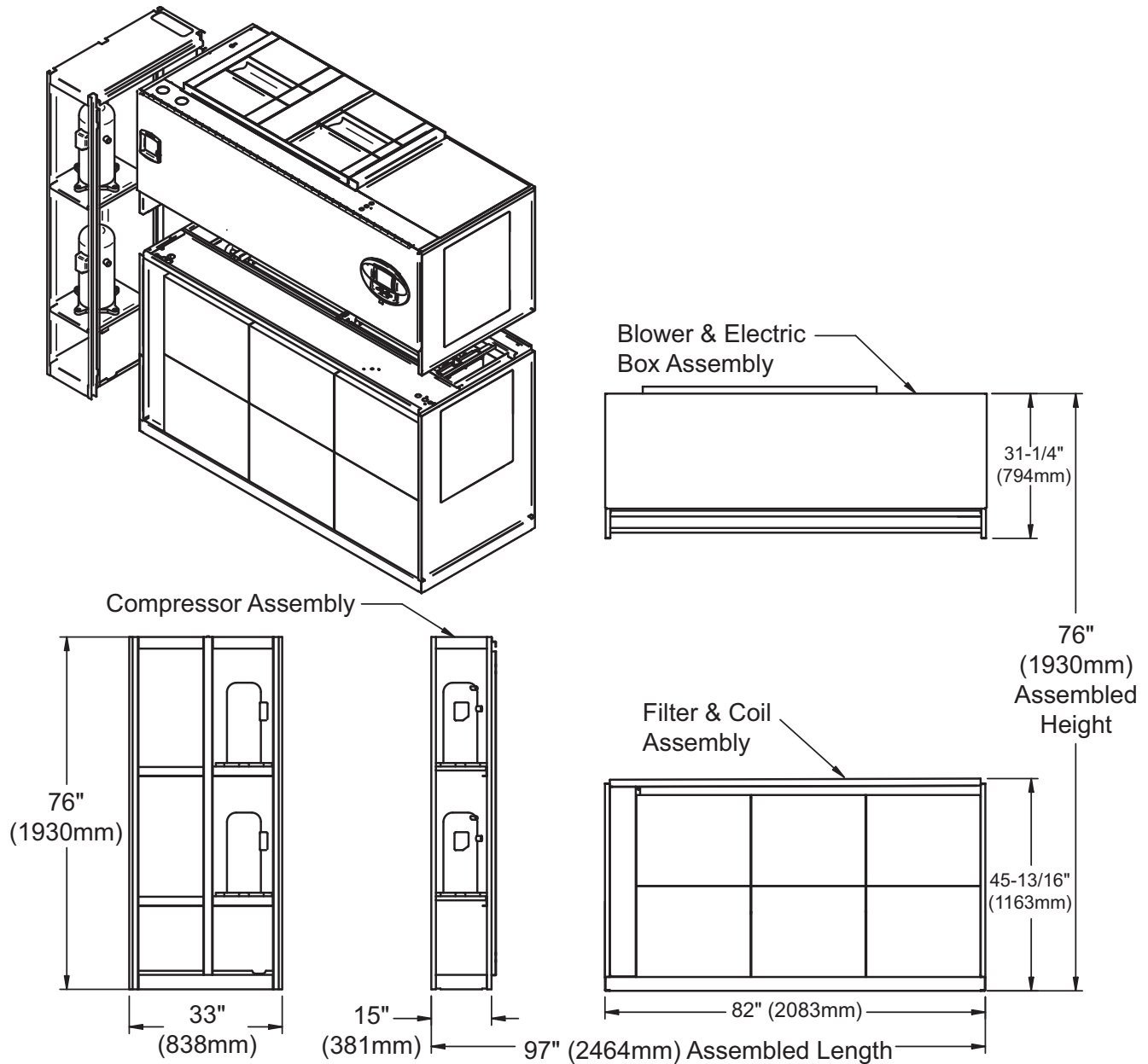
Figure 56 Component dimensions—upflow, air-cooled, 53-77kw (15-22 ton), scroll/digital scroll compressor models
