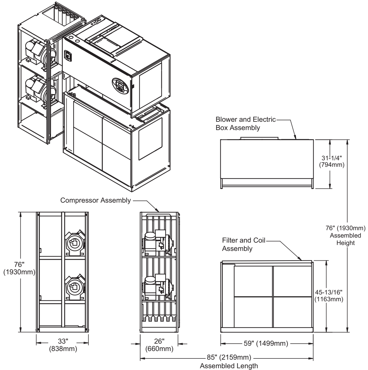
Figure 54 Component dimensions—upflow, water/glycol/GLYCOOL, 28-42kW (8-12 ton), all compressor models
