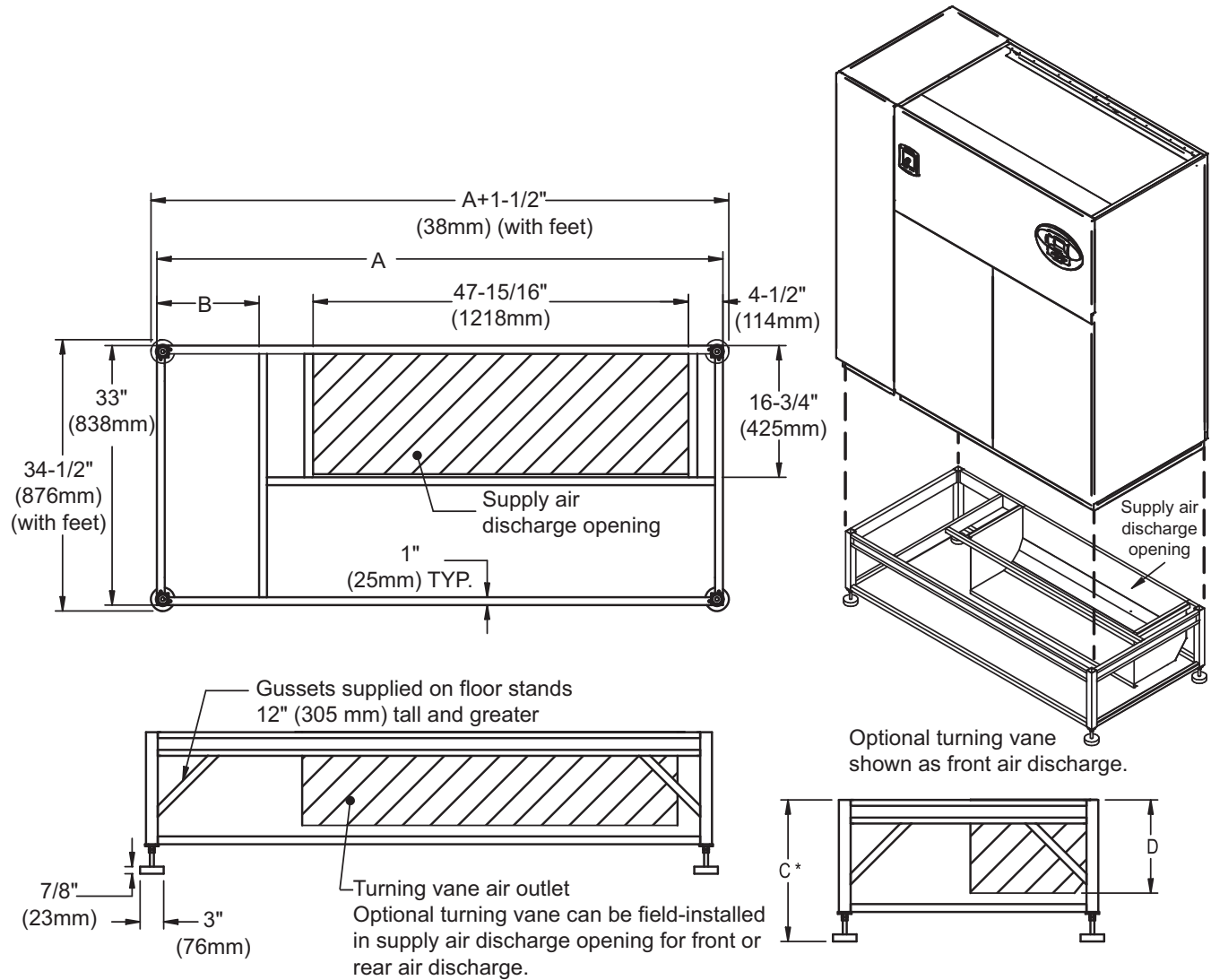
Figure 22 Floor stand dimensions—downflow, 28-42kW (8-12 ton) models
