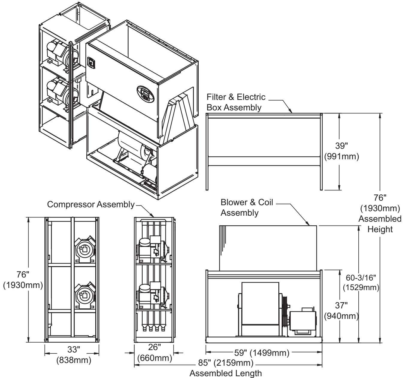
Figure 45 Component dimensions—downflow, water/glycol/GLYCOOL, 28-42kW (8-12 ton), all compressor models
