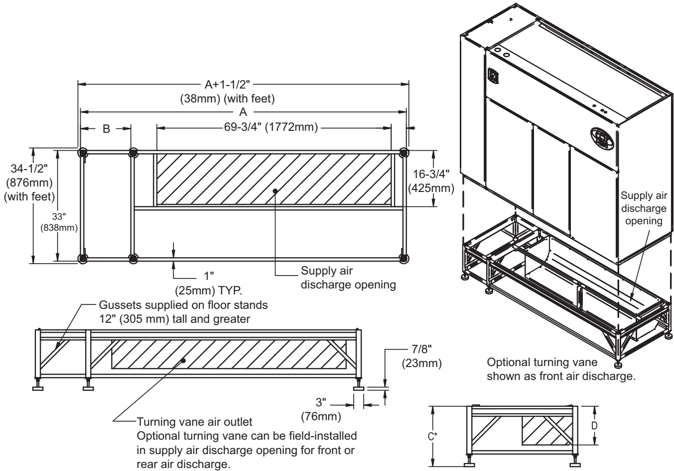
Figure 23 Floor stand dimensions—downflow, 53-77kW (15-22 ton) models
