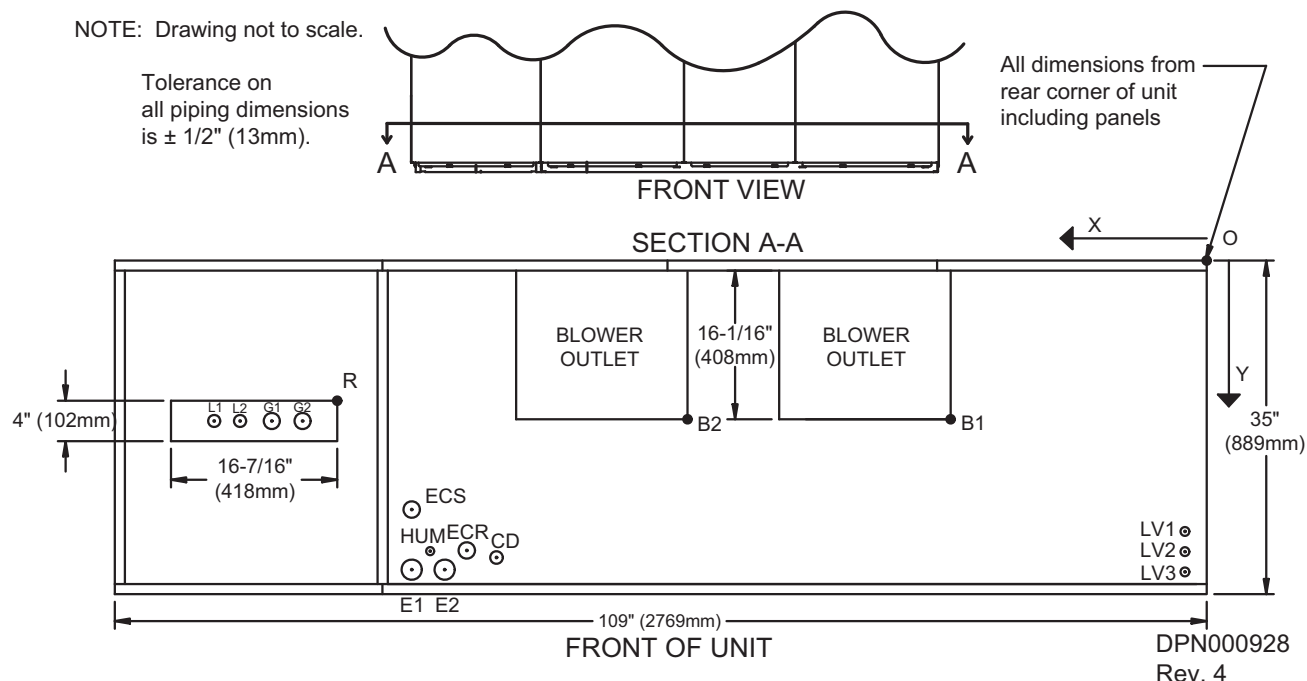
Figure 80 Primary connection locations—downflow, air-Cooled, 53-77kW (15-22 ton), semi-hermetic compressor models
