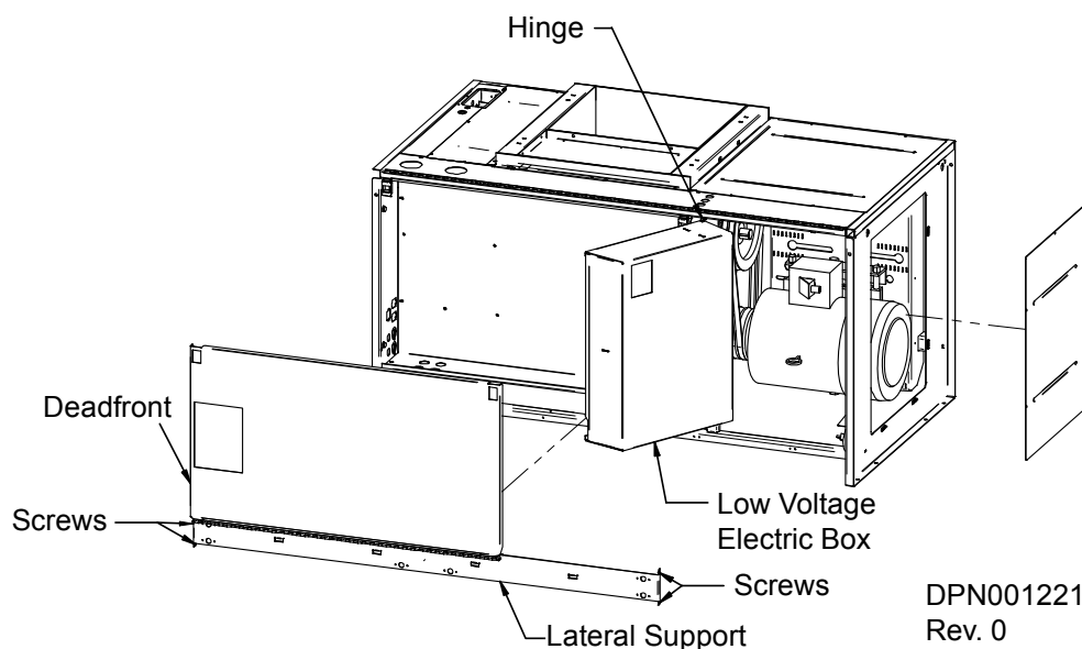
Figure 99 Upflow motor access
