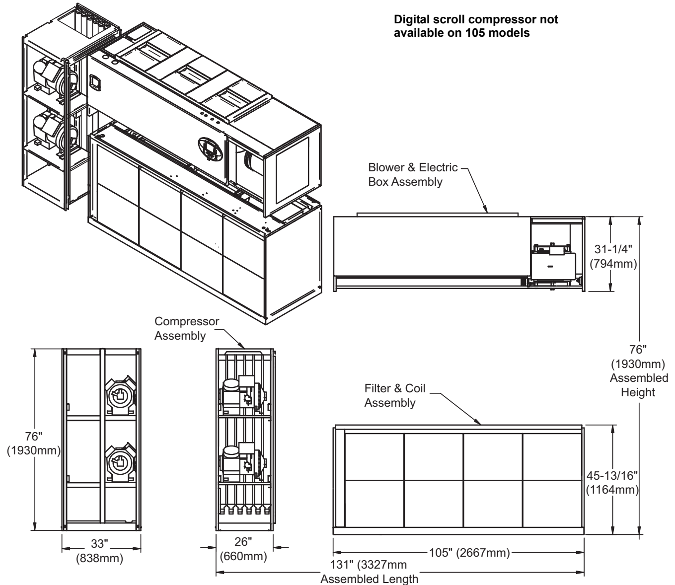
Figure 60 Component dimensions—upflow, water/glycol/GLYCOOL, 105kW (30 ton), all compressor models
