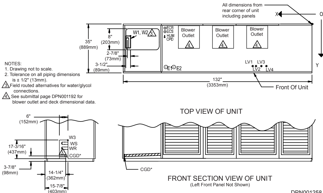
LEFT SIDE SECTION VIEW OF UNIT
