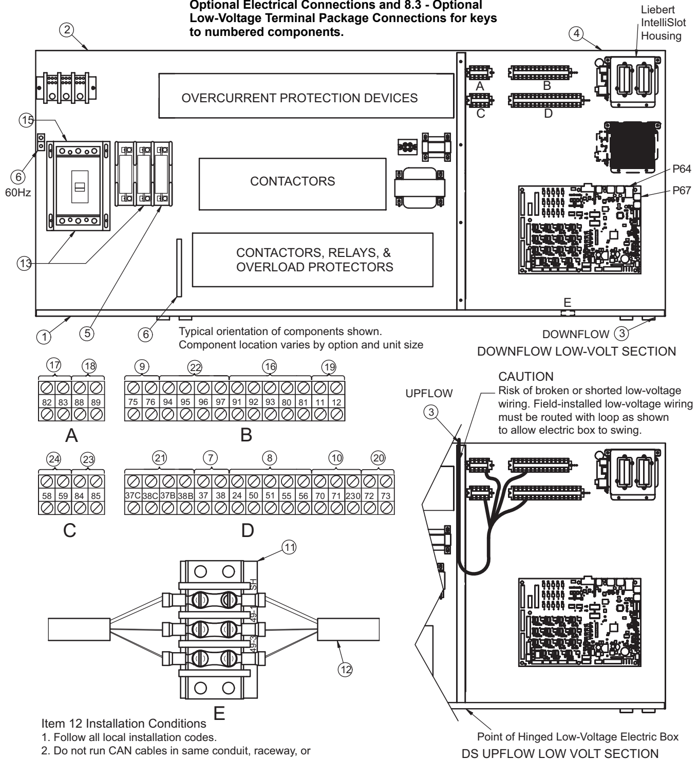
Figure 61 Electrical field connections—Upflow and downflow models, single molded case switch disconnect with main fuses
