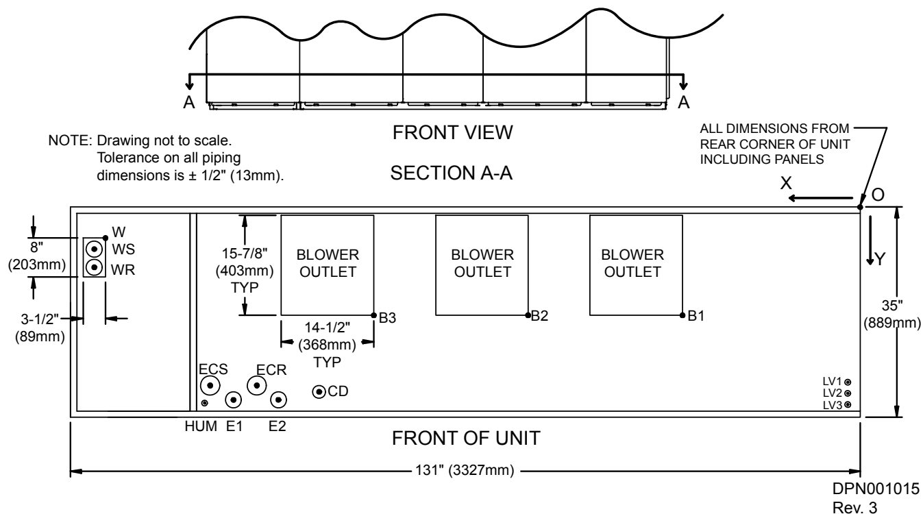
Figure 88 Primary connection locations—downflow, water/glycol/GLYCOOL, 105kW (30 ton), all compressor *** models
