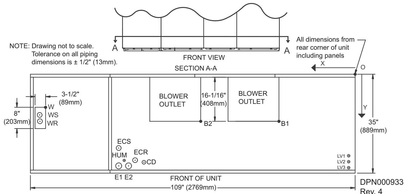
Figure 84 Primary connection locations—downflow, water/glycol/GLYCOOL, 53-77kW (15-22 ton), all compressor *** models
