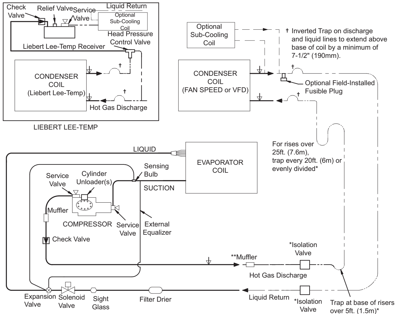
Figure 68 Piping schematic—air-cooled, semi-hermetic compressor models
