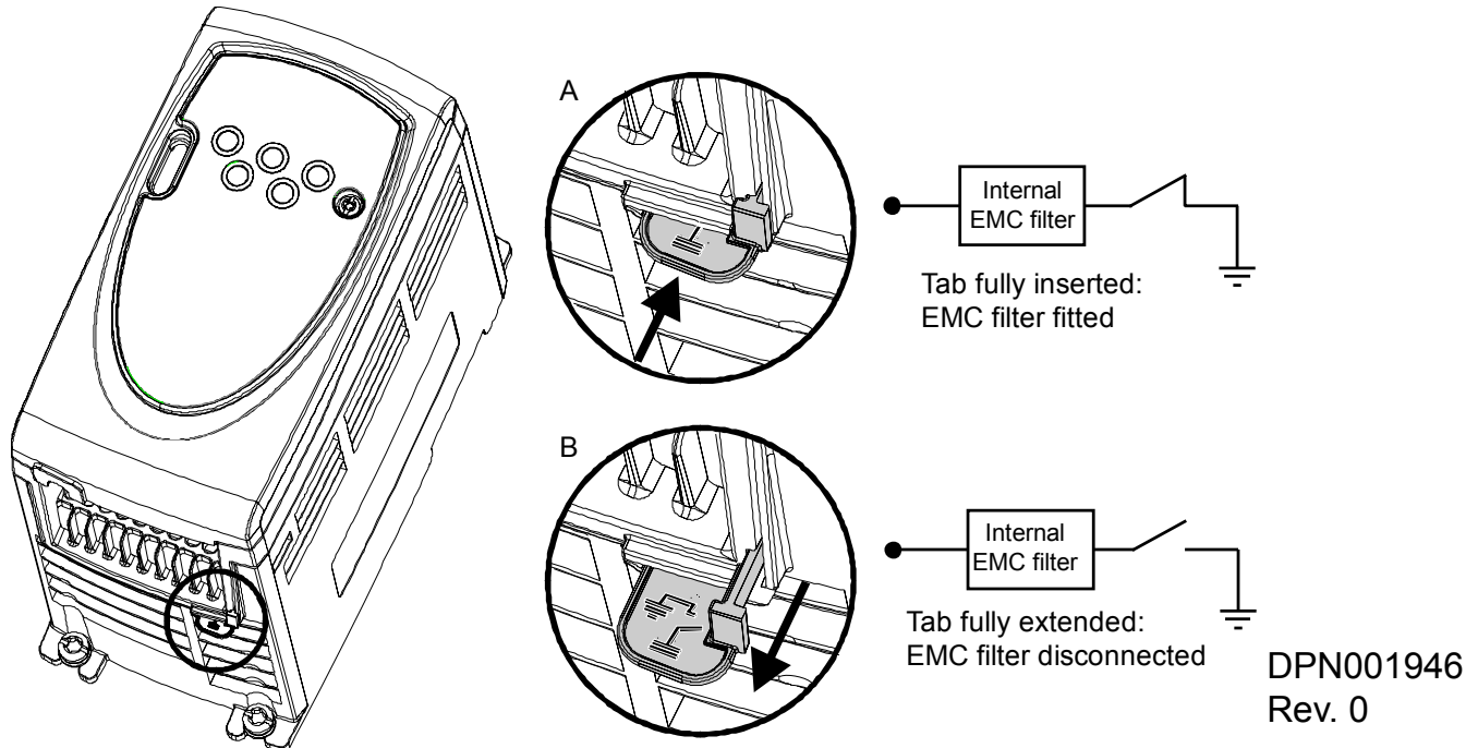
Figure 65 Disconnecting EMC filter for operation with Delta-connected power size C & D inverters
