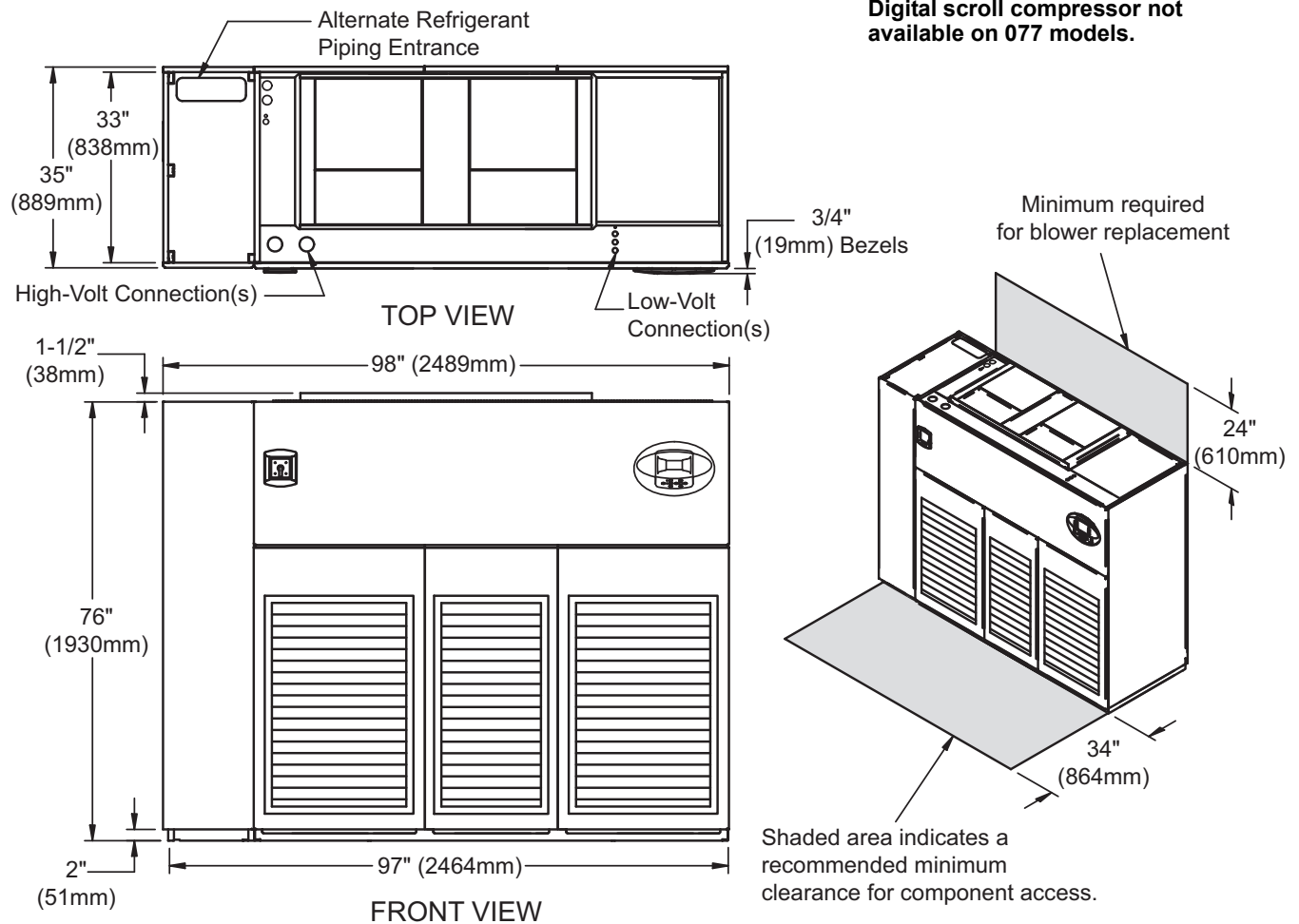
Figure 18 Cabinet and floor planning dimensions—upflow, air-cooled, 53-77kW (15-22 ton), scroll or digital scroll compressor models
