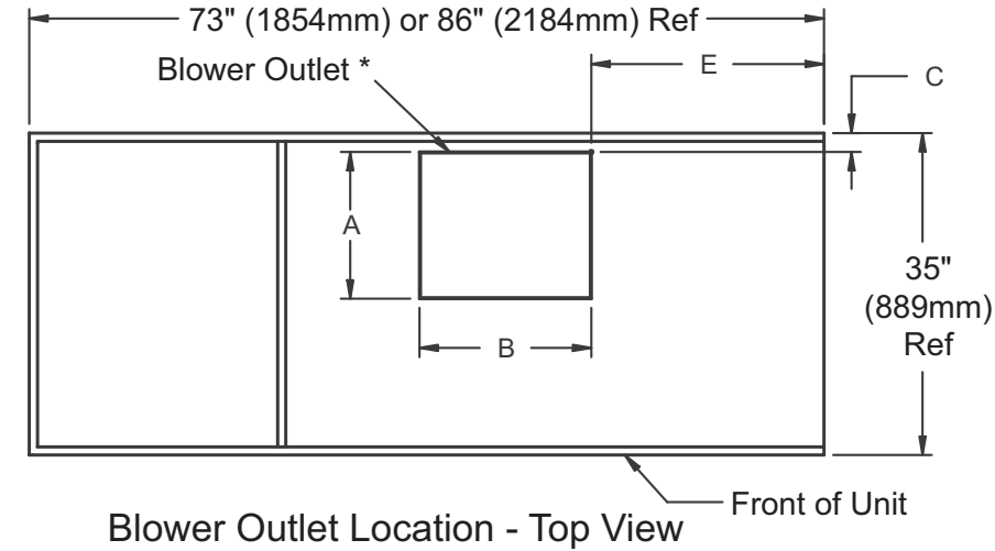
Figure 27 Blower outlet and deck dimensions—upflow, 28-42kW (8-12 ton)
