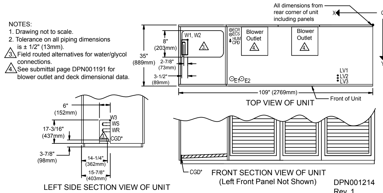
Figure 95 Primary connection locations—upflow, water/glycol/GLYCOOL, 53-77kW (15-22 ton), all compressor *** models
