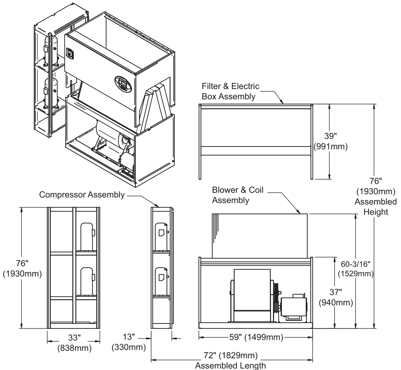
Figure 44 Component dimensions—downflow, air-cooled, 28-42kW (8-12 ton), scroll/digital scroll compressor models
