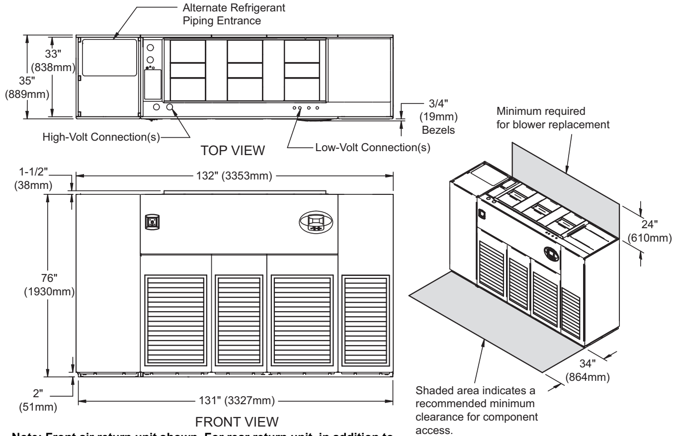
Figure 20 Cabinet and floor planning dimensions—upflow, air-cooled, 105kW (30 ton), all models
