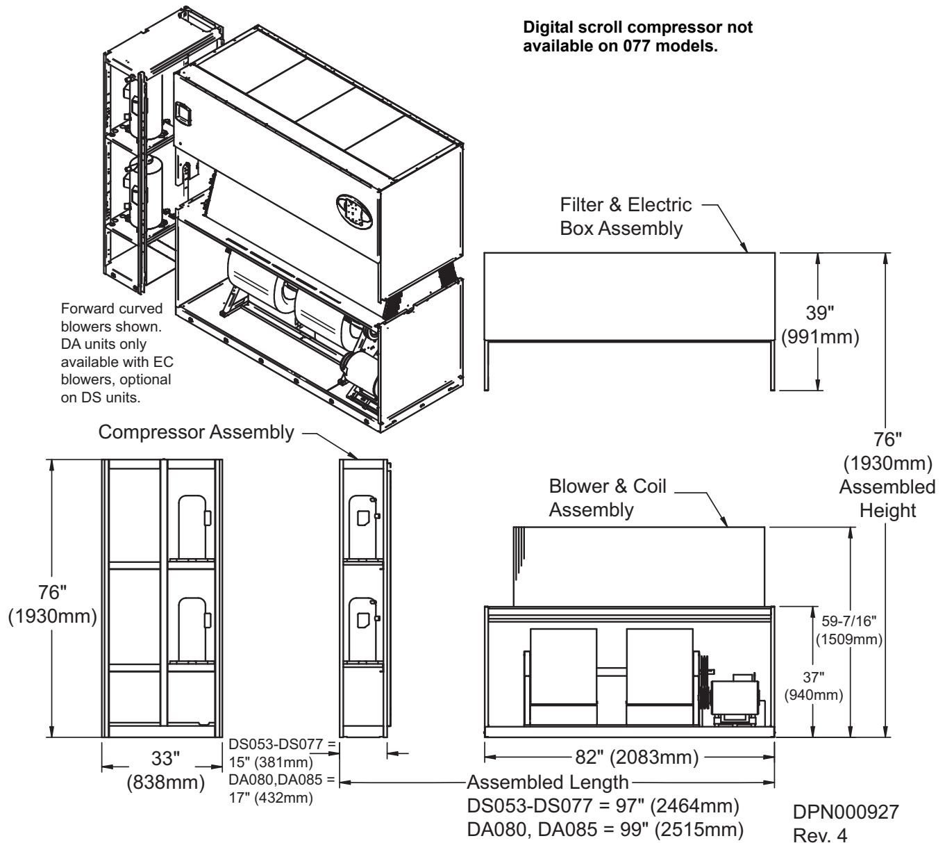
Figure 47 Component dimensions—downflow air-cooled, 53-77kW (15-22 ton), scroll/digital scroll compressor models; forward-curved and EC fan
