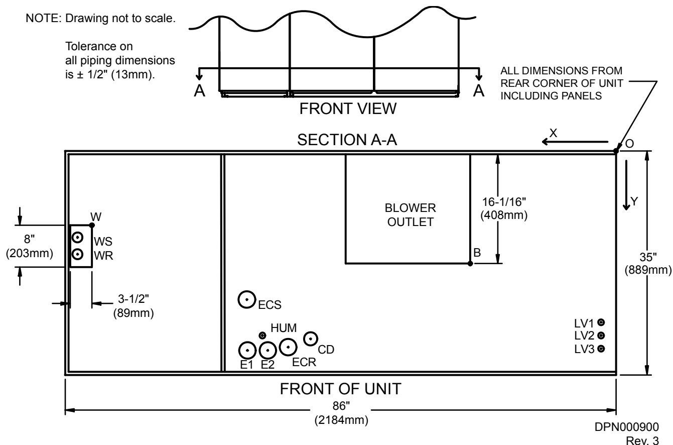
Figure 79 Primary connection locations—downflow water/glycol/GLYCOOL 28-42kW (8-12 ton), all compressor models
