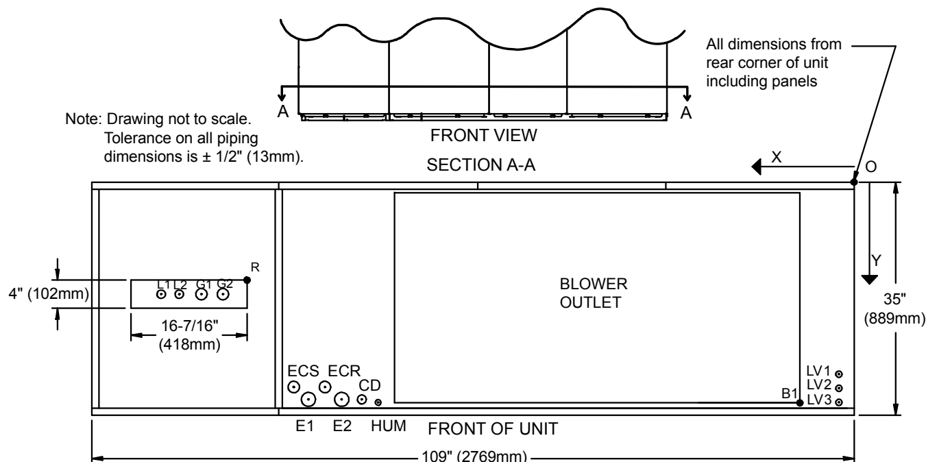
Figure 81 Primary connection locations downflow air cooled 53-77kW (15-22 tons) semi-hermetic compressor models, with EC fans
