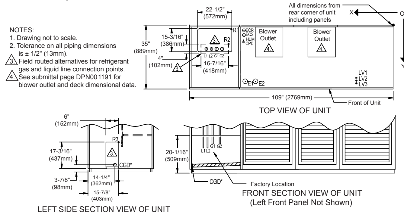
Figure 93 Primary connection locations—upflow, air-cooled, 53-77kW (15-22 ton), semi-hermetic compressor models
