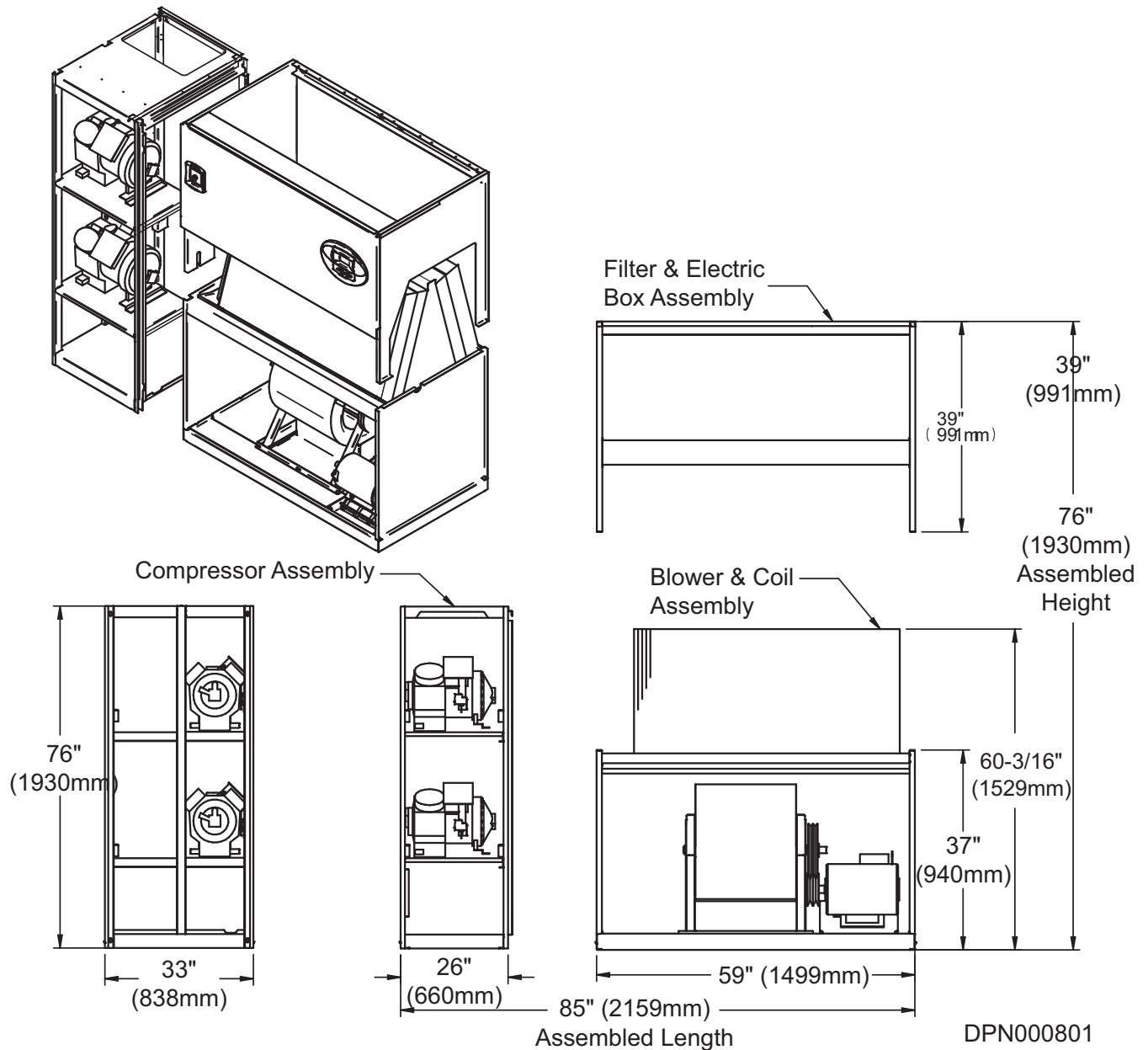
Figure 43 Component dimensions—downflow, air-cooled, 28-42kW (8-12 ton), semi-hermetic compressor models
