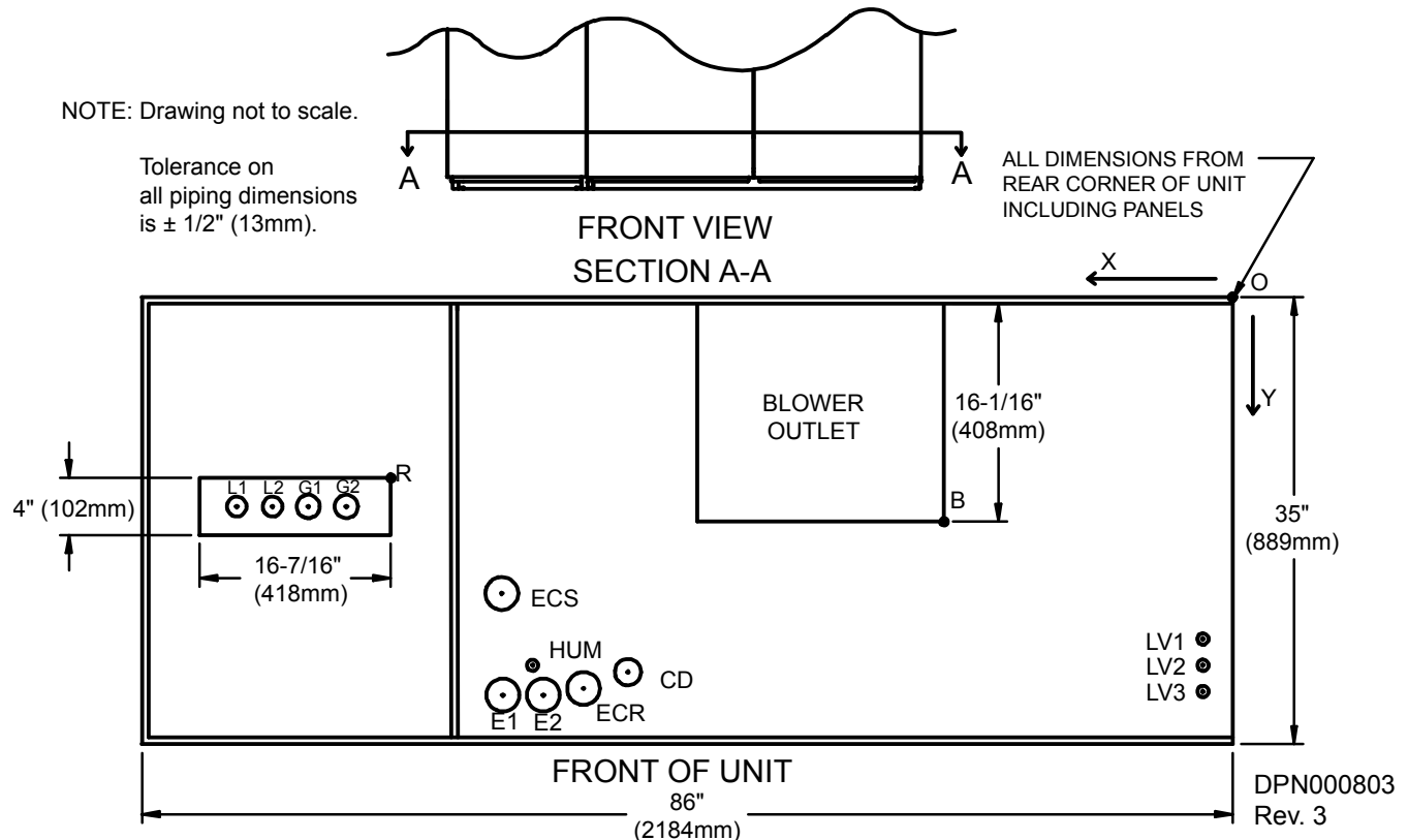
Figure 77 Primary connection locations—downflow, air-cooled, 28-42kW (8-12 ton), semi-hermetic compressor models
