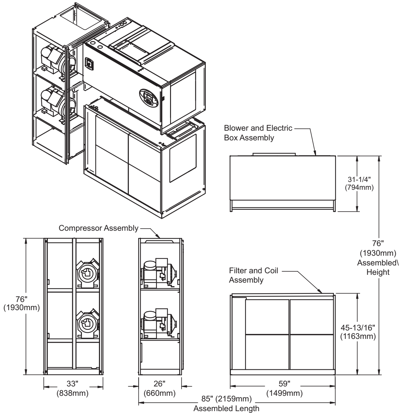
Figure 52 Component dimensions—upflow, air-cooled, 28-42kW (8-12 ton), semi-hermetic compressor models
