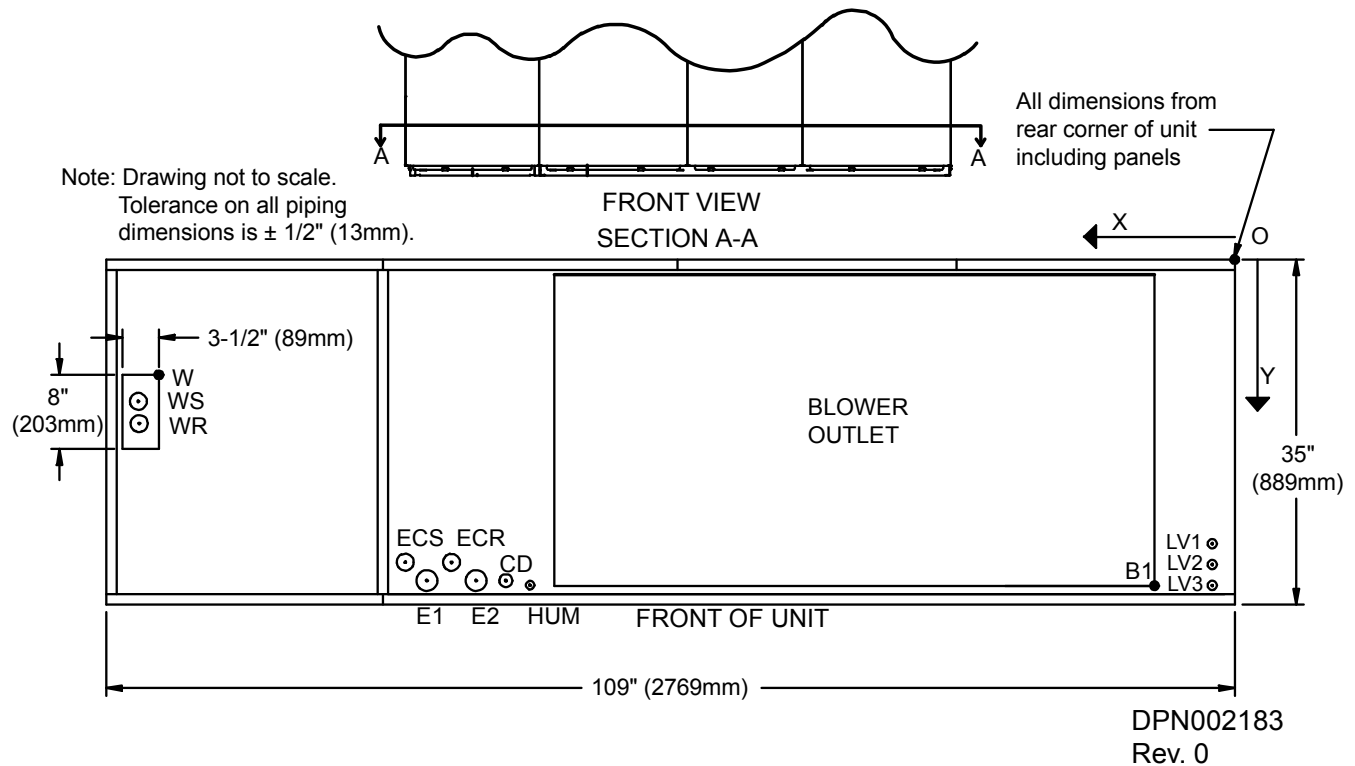
Figure 85 Primary connection locations—downflow, water/glycol/GLYCOOL, 53-77kW (15-22 ton), all compressor *** models, with EC fans
