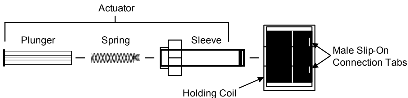
Figure 105 Drain valve assembly
