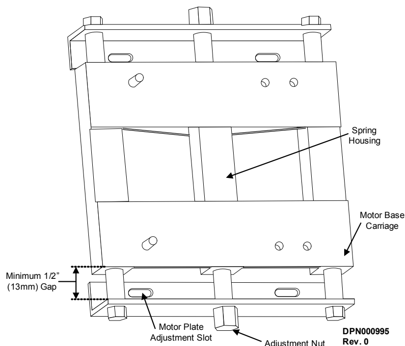
Figure 100 Auto-belt tensioning motor base
