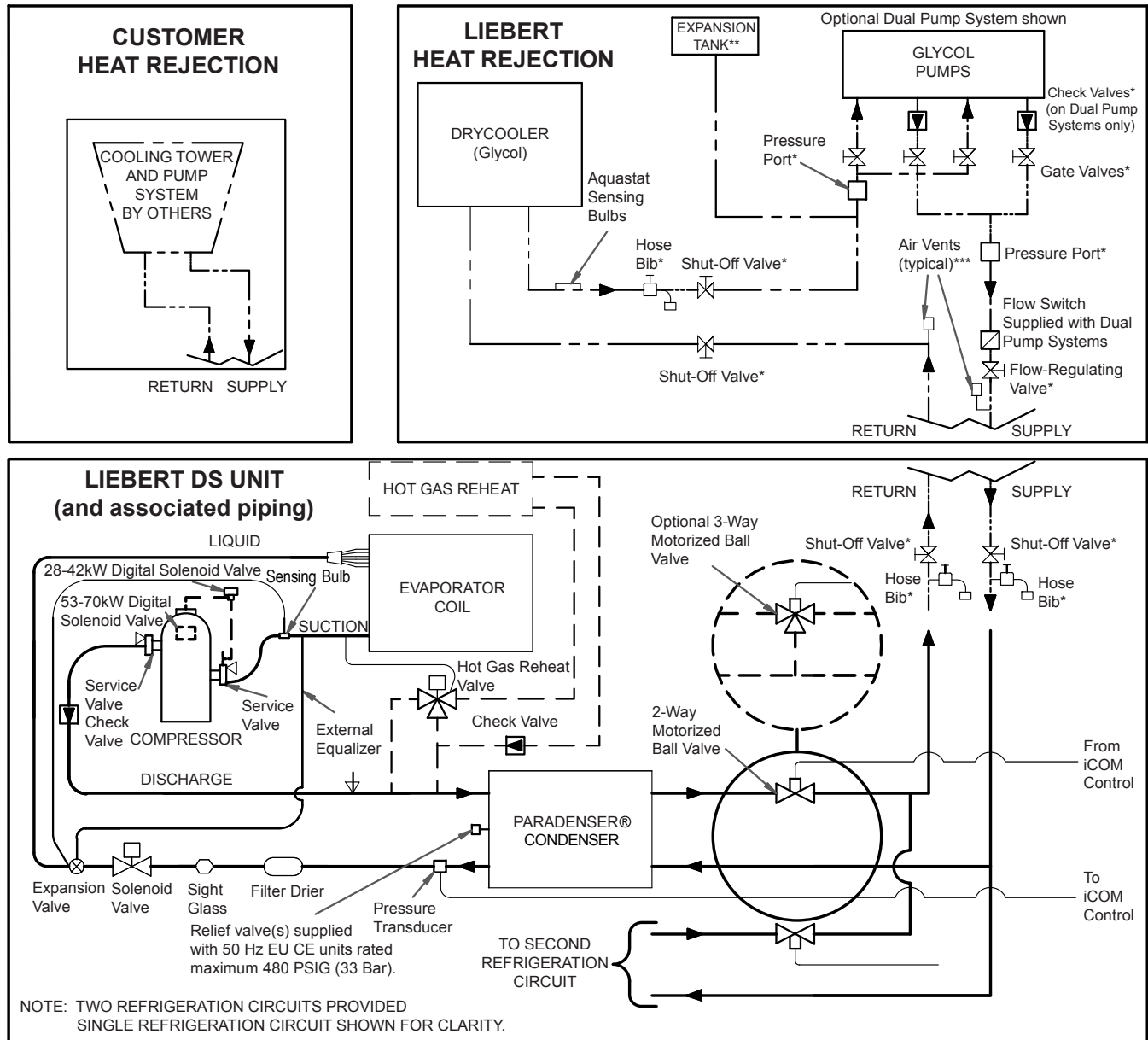
Figure 74 Piping schematic—water/glycol with digital scroll compressor models
