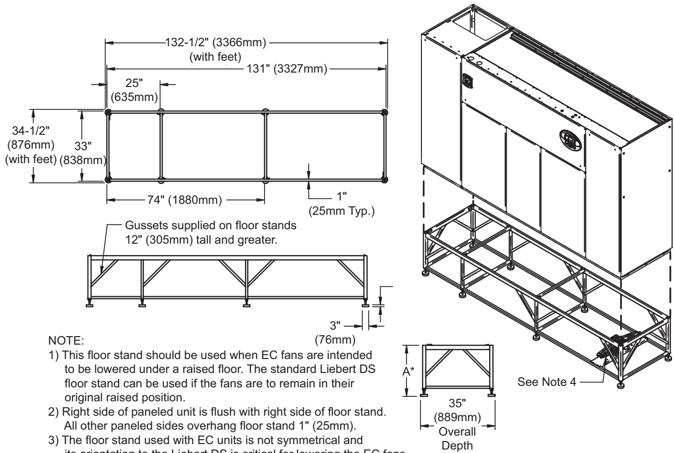
Figure 26 Floor stand and floor planning dimension, downflow 105kW (30 tons) models with EC fans
