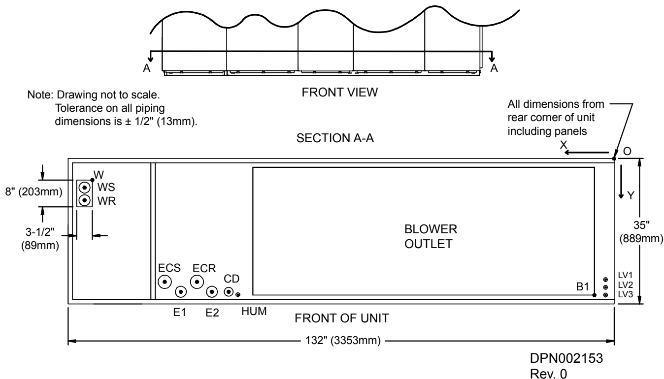
Figure 89 Primary connection locations downflow water/glycol/GLYCOOL 105kW (30 tons) all compressor *** models, with EC fan
