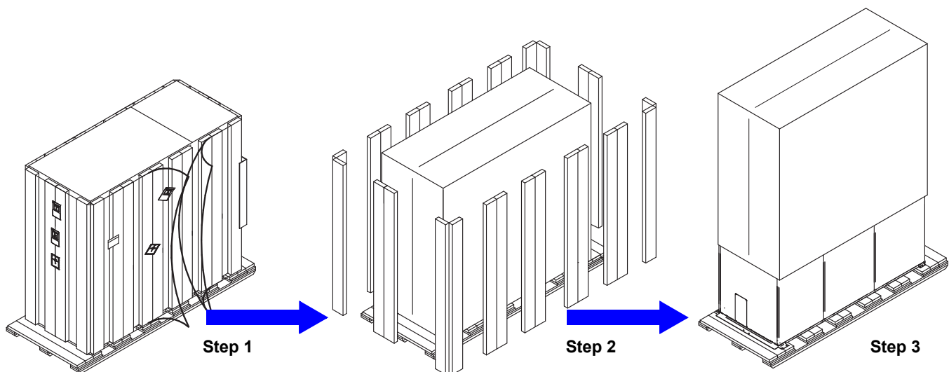
Figure 33 Removing packaging
