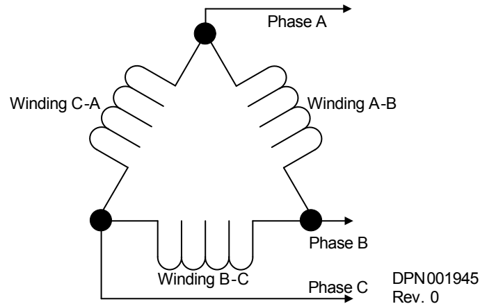
Figure 64 Delta-connected power diagram
