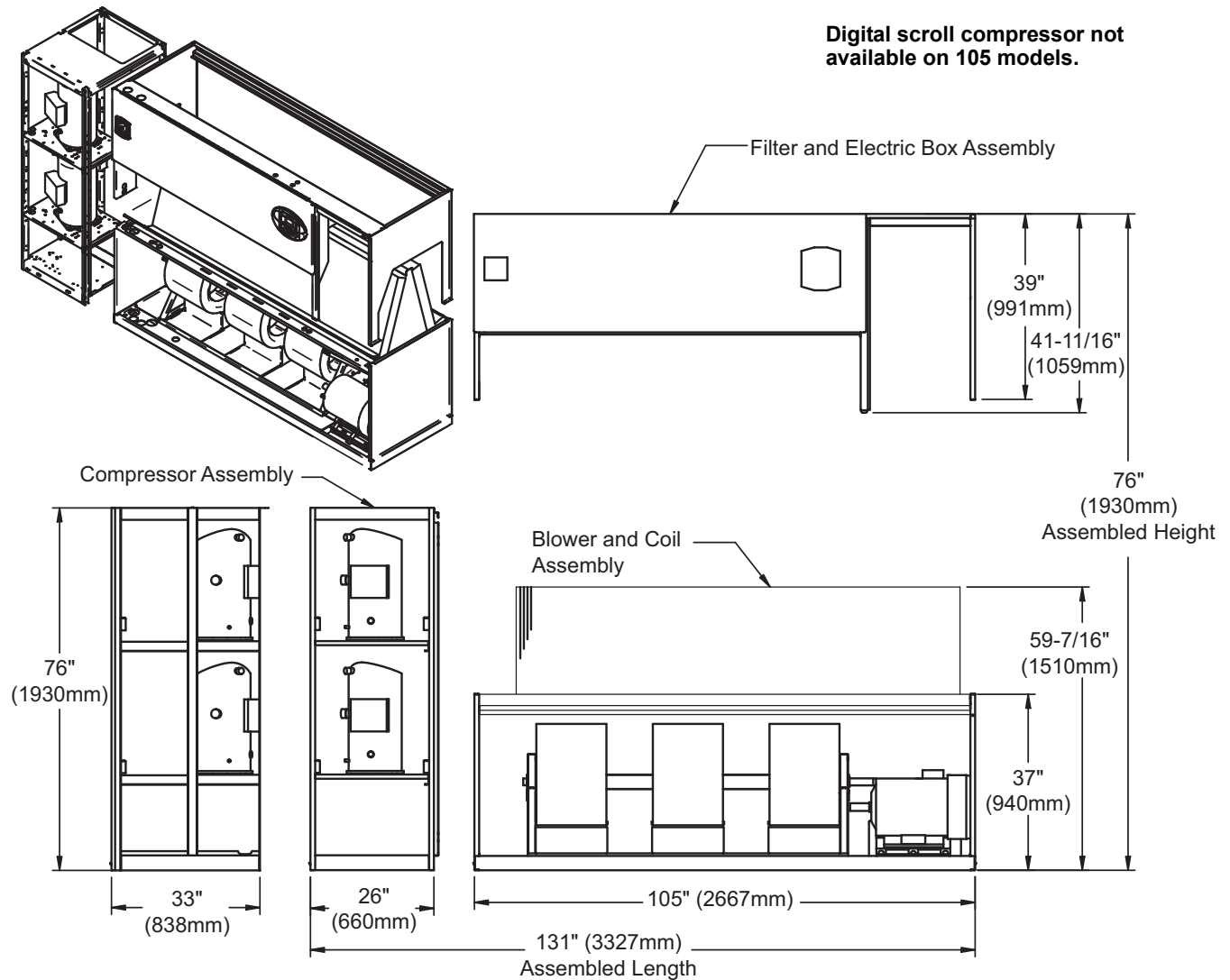
Figure 50 Component dimensions—downflow, air-cooled, 105kW (30 ton), scroll compressor models; forward-curved and EC fan
