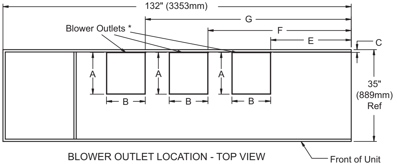
Figure 29 Blower outlet and deck dimensions—upflow 105kW (30ton)
