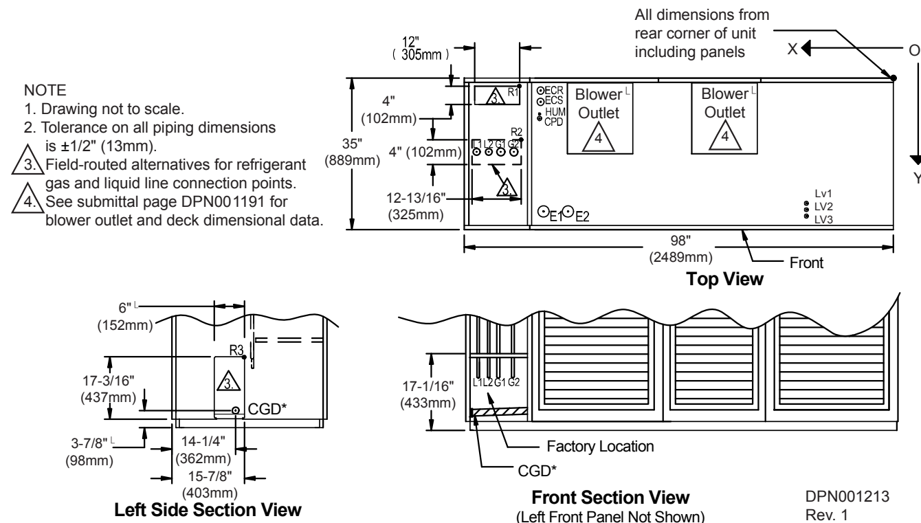
Figure 94 Primary connection locations—upflow, air-cooled, 53-77kW (15-22 ton), scroll compressor *** models
