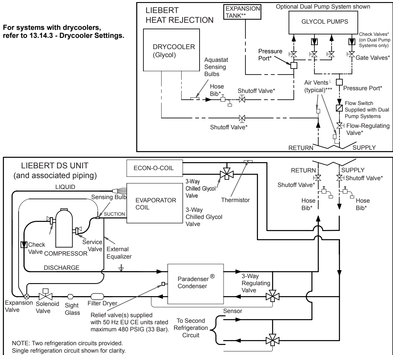
Figure 73 Piping schematic—GLYCOOL with scroll compressor models
