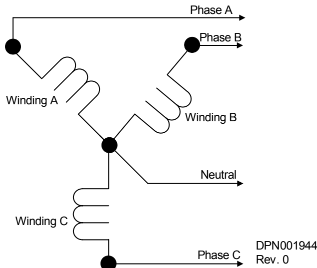
Figure 63 Wye-connected power diagram
