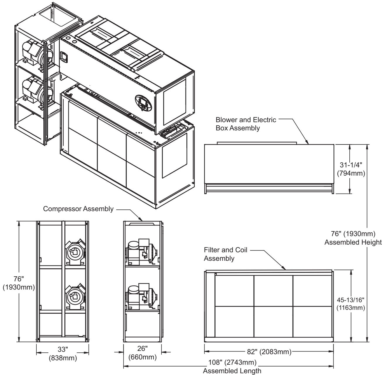
Figure 55 Component dimensions—upflow, air-cooled, 53-77kw (15-22 ton), semi-hermetic compressor models
