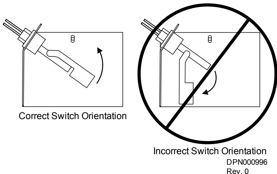
Figure 101 Correct orientation of float switch
