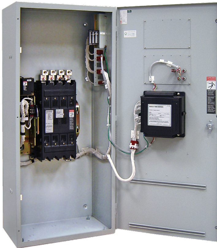
Four Pole, Non-Automatic, Electrically-Operated 400 Amp Switch in a Type 1 Enclosure
